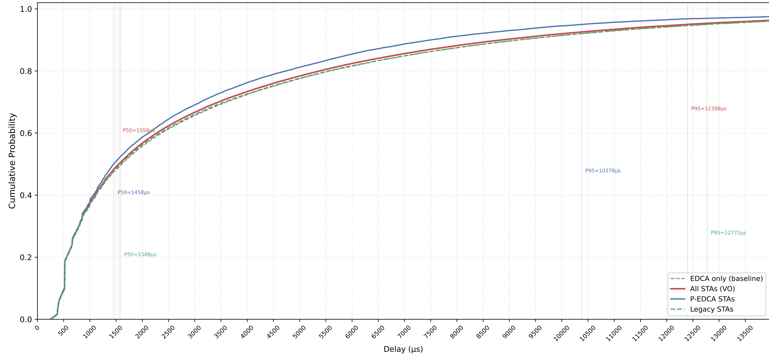
VO Delay CDF — P-EDCA / Legacy / All | CWds=1 × QSRC=3 × PSRC=3 nSta=30, nPedca=5/30, 1Mbps, avg of 10 runs
