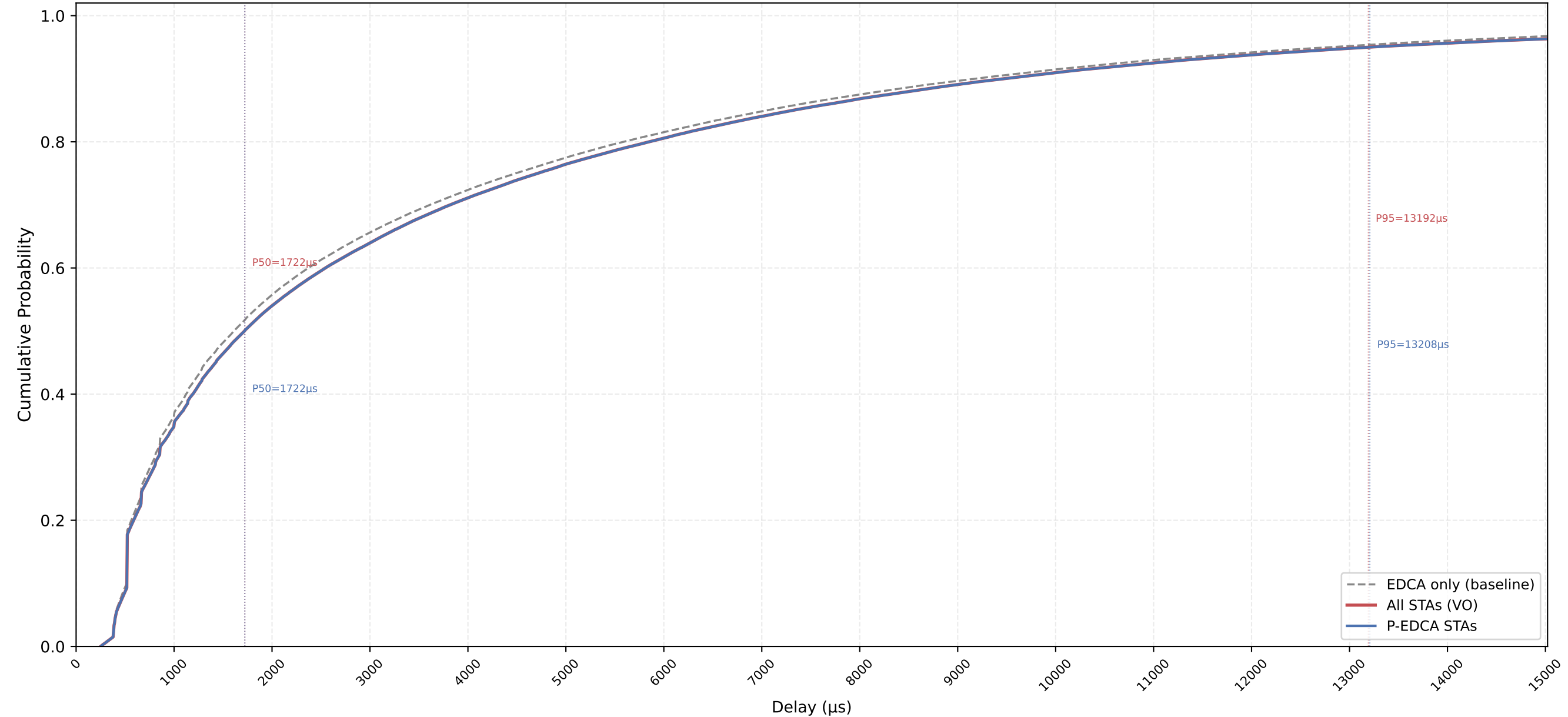
VO Delay CDF — P-EDCA / Legacy / All | CWds=1 × QSRC=4 × PSRC=1 nSta=30, nPedca=30/30, 1Mbps, avg of 10 runs
