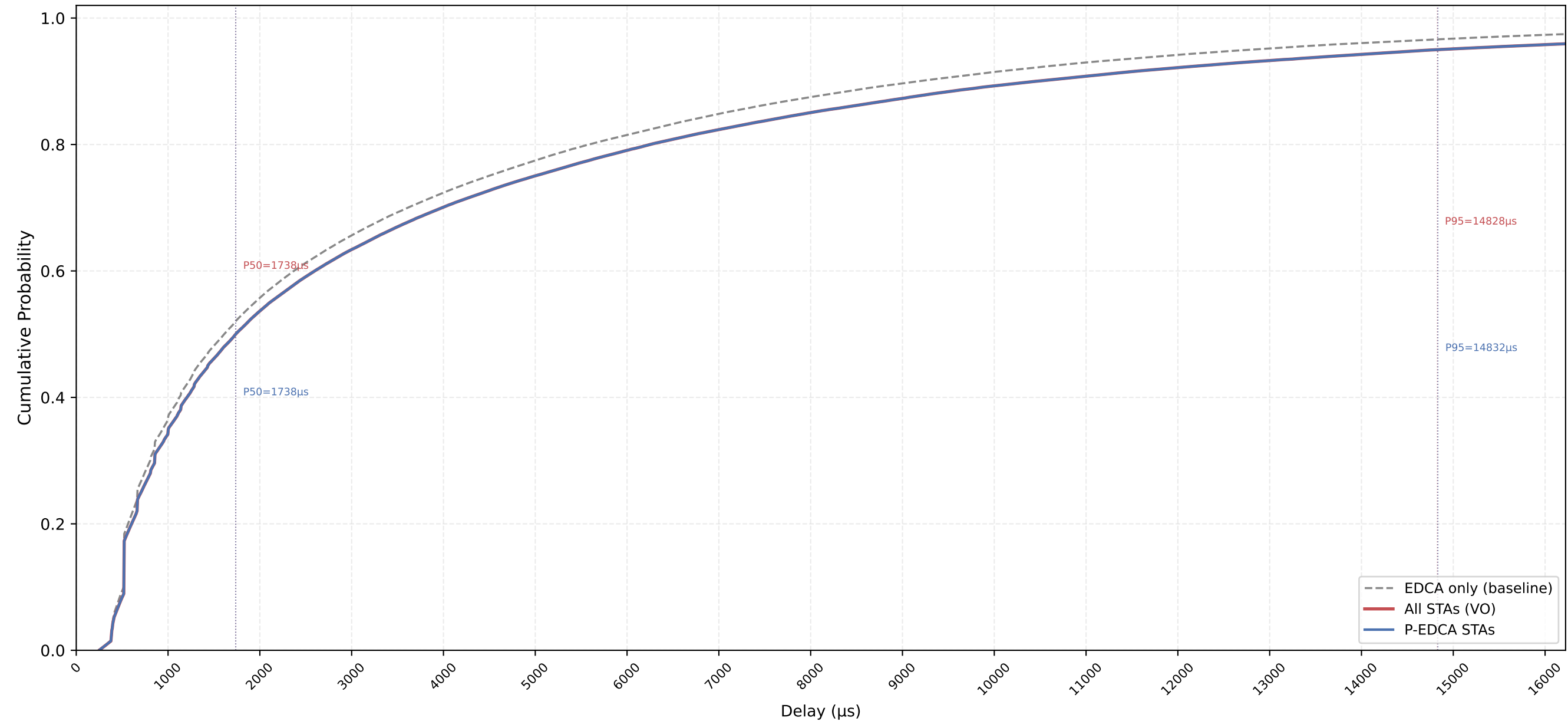
VO Delay CDF — P-EDCA / Legacy / All | CWds=1 × QSRC=5 × PSRC=2 nSta=30, nPedca=30/30, 1Mbps, avg of 10 runs
