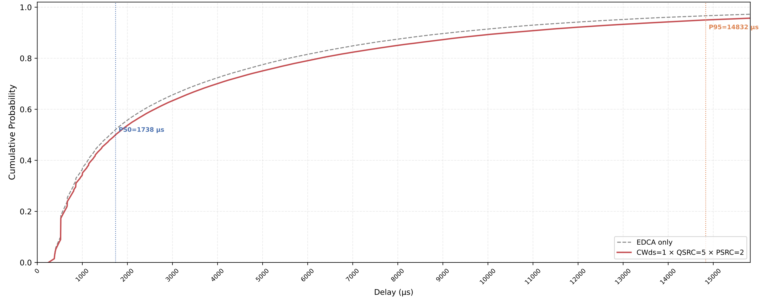
P-EDCA STA VO Delay CDF — CWds=1 × QSRC=5 × PSRC=2 nSta=30, nPedca=30, 1Mbps, avg of 10 runs
