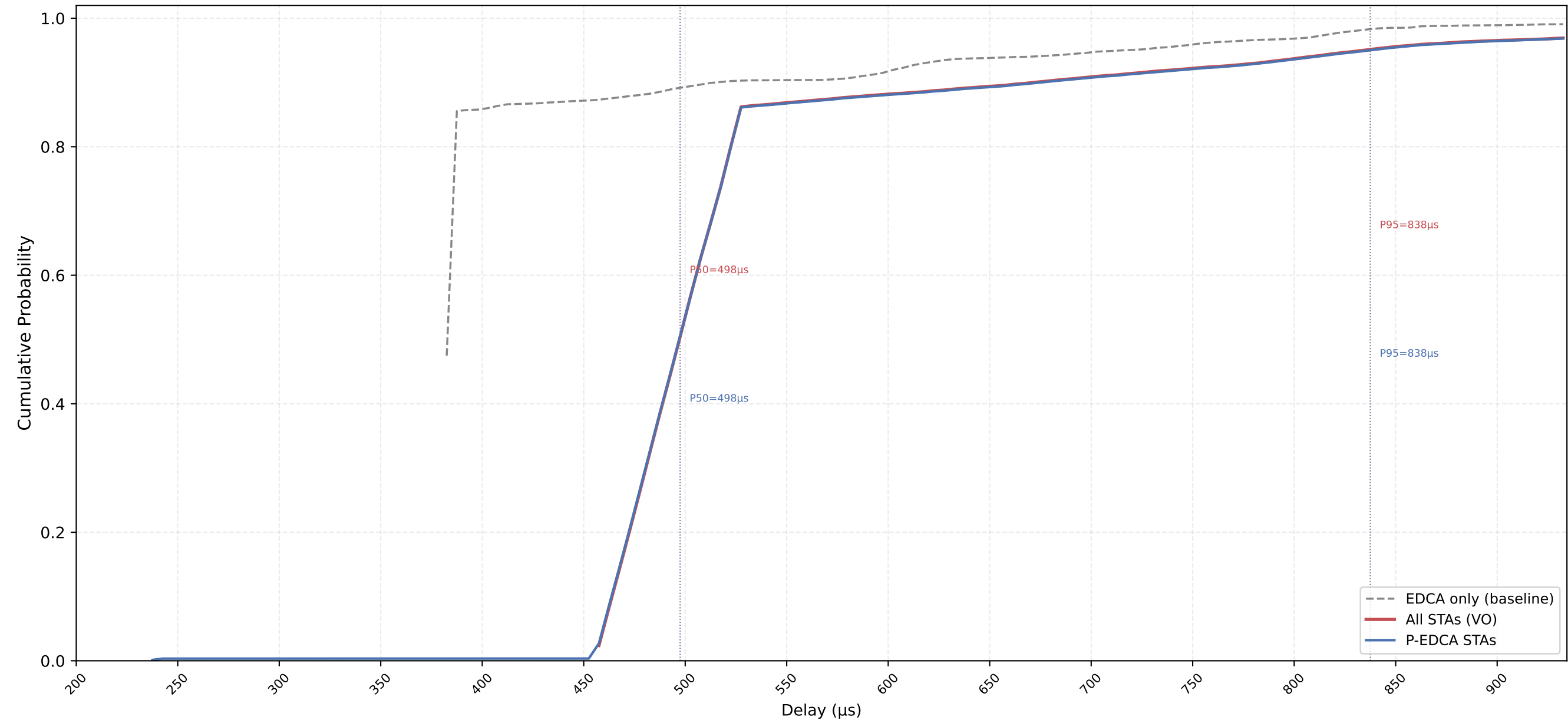
VO Delay CDF — P-EDCA / Legacy / All | CWds=0 × QSRC=0 × PSRC=1 nSta=30, nPedca=30/30, 0.1Mbps, avg of 10 runs
