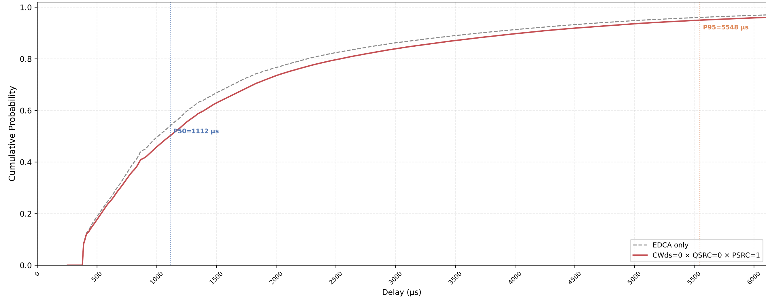
Legacy STA VO Delay CDF — CWds=0 × QSRC=0 × PSRC=1 nSta=30, nPedca=5, 0.5Mbps, avg of 10 runs
