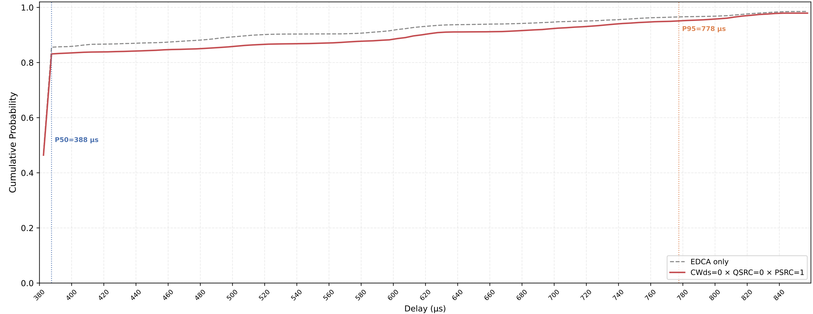
Legacy STA VO Delay CDF — CWds=0 × QSRC=0 × PSRC=1 nSta=30, nPedca=15, 0.1Mbps, avg of 10 runs
