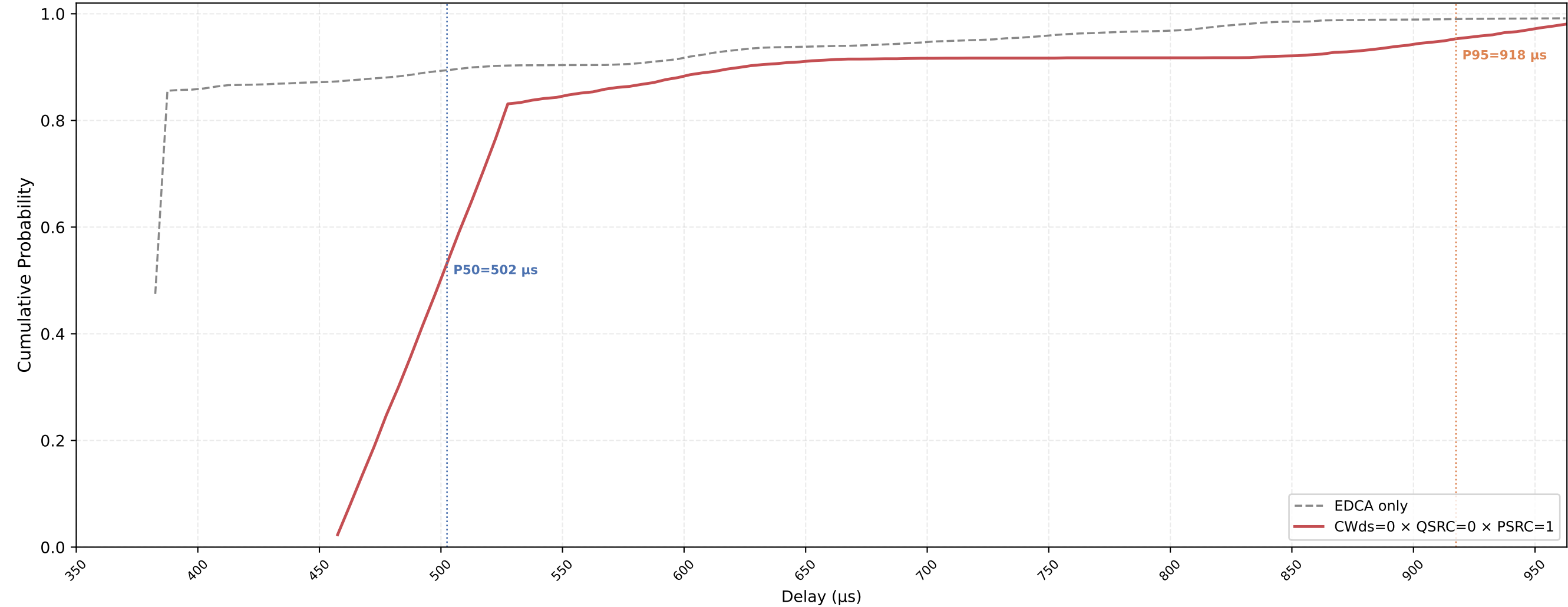
P-EDCA STA VO Delay CDF — CWds=0 × QSRC=0 × PSRC=1 nSta=30, nPedca=5, 0.1Mbps, avg of 10 runs
