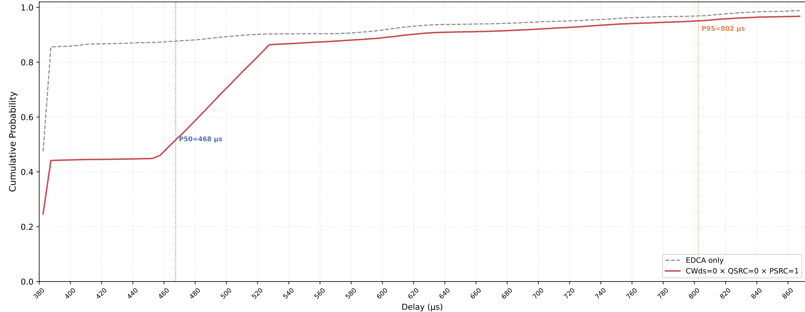
VO (all STAs) Delay CDF — CWds=0 × QSRC=0 × PSRC=1 nSta=30, nPedca=15, 0.1Mbps, avg of 10 runs
