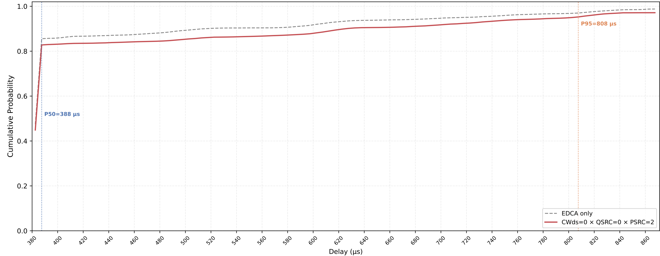
Legacy STA VO Delay CDF — CWds=0 × QSRC=0 × PSRC=2 nSta=30, nPedca=15, 0.1Mbps, avg of 10 runs
