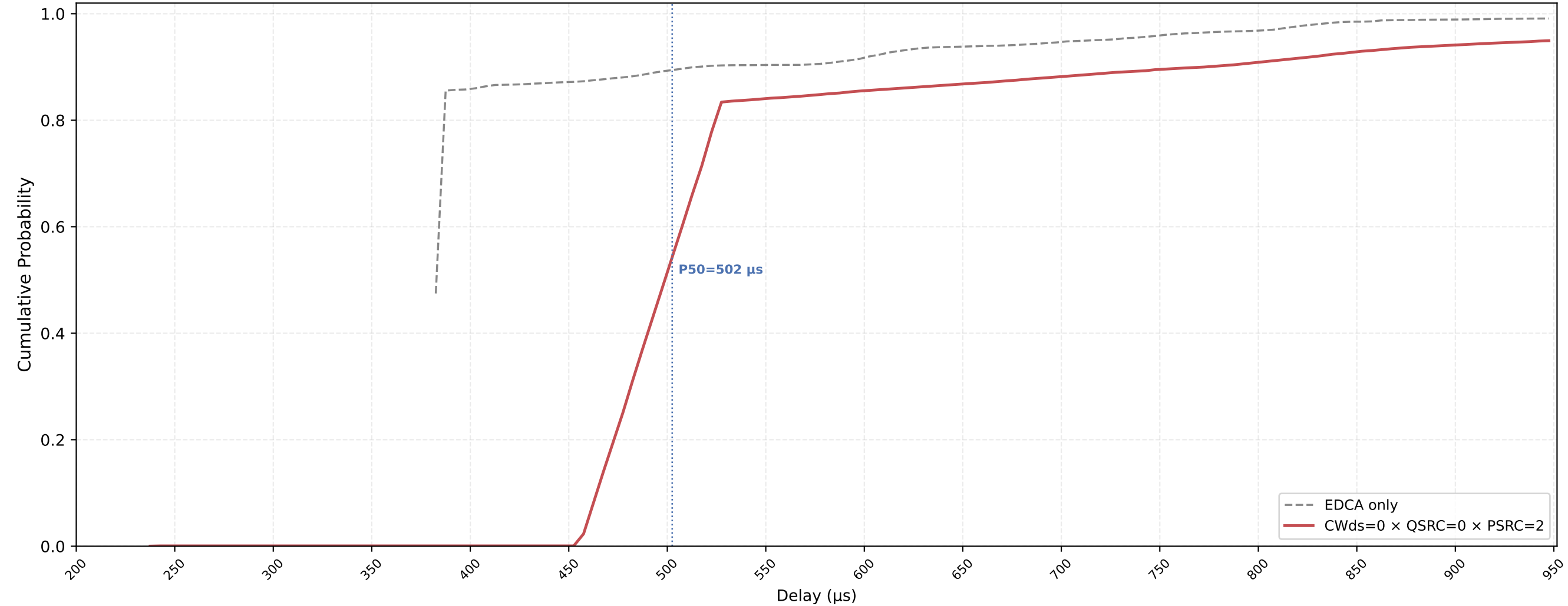
P-EDCA STA VO Delay CDF — CWds=0 × QSRC=0 × PSRC=2 nSta=30, nPedca=30, 0.1Mbps, avg of 10 runs
