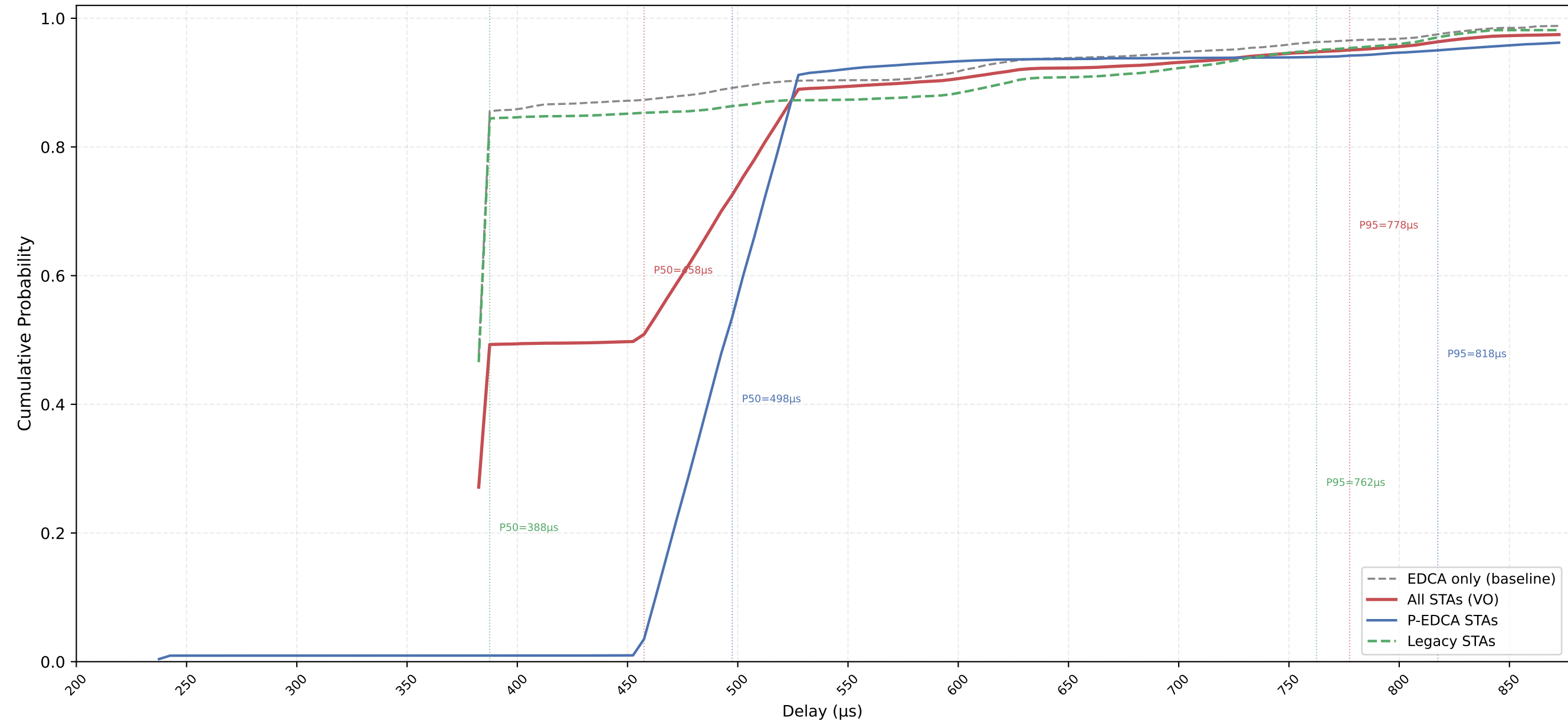
VO Delay CDF — P-EDCA / Legacy / All | CWds=0 × QSRC=0 × PSRC=3 nSta=30, nPedca=15/30, 0.1Mbps, avg of 10 runs
