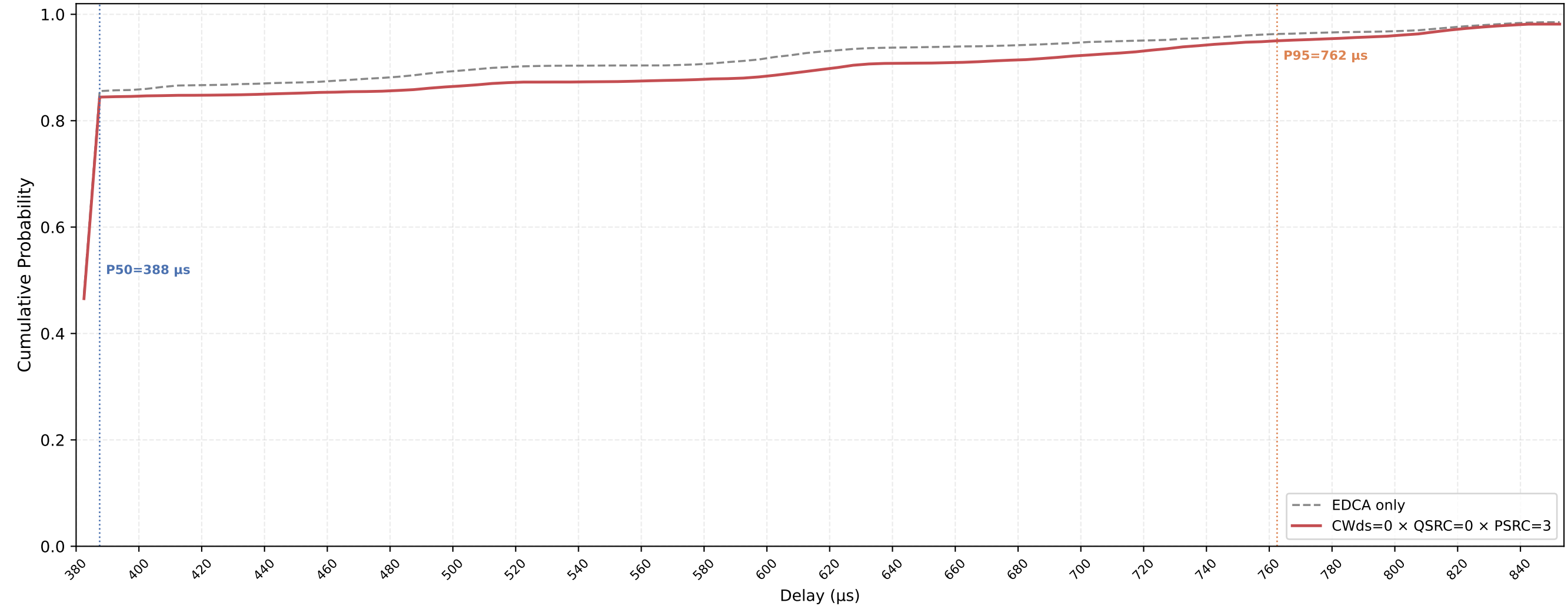
Legacy STA VO Delay CDF — CWds=0 × QSRC=0 × PSRC=3 nSta=30, nPedca=15, 0.1Mbps, avg of 10 runs
