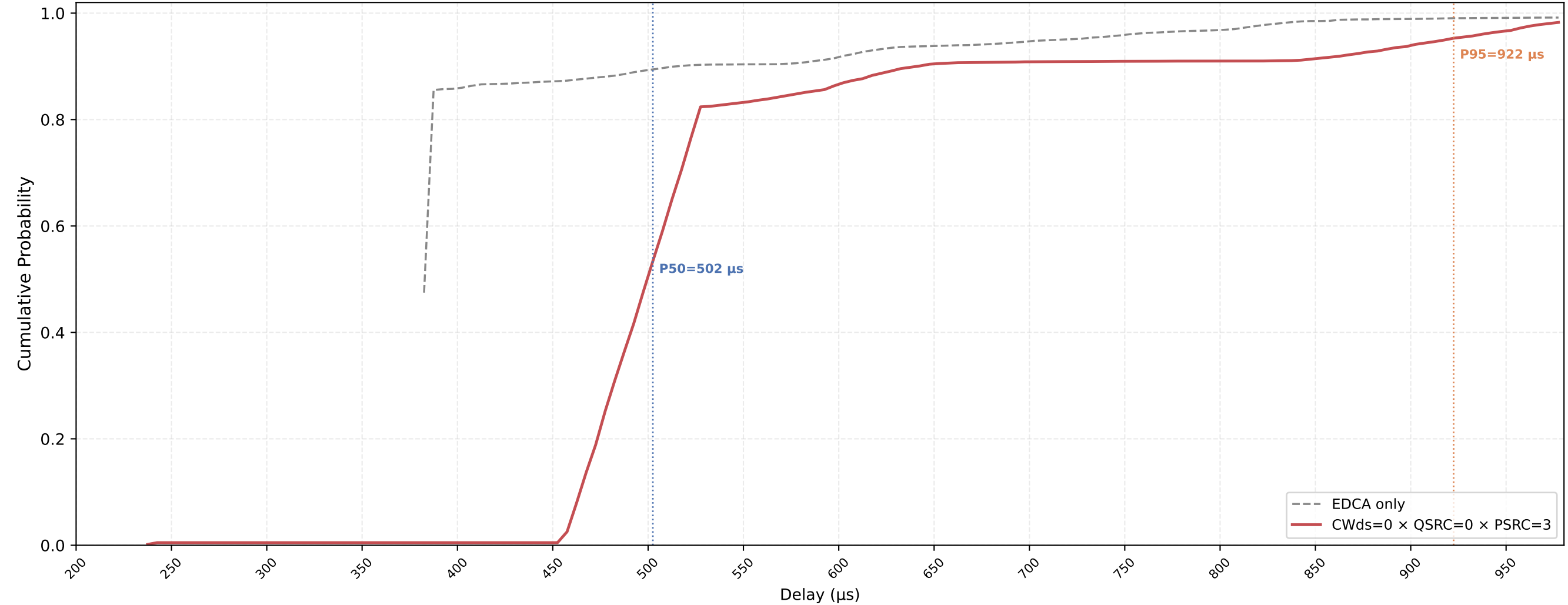
P-EDCA STA VO Delay CDF — CWds=0 × QSRC=0 × PSRC=3 nSta=30, nPedca=5, 0.1Mbps, avg of 10 runs
