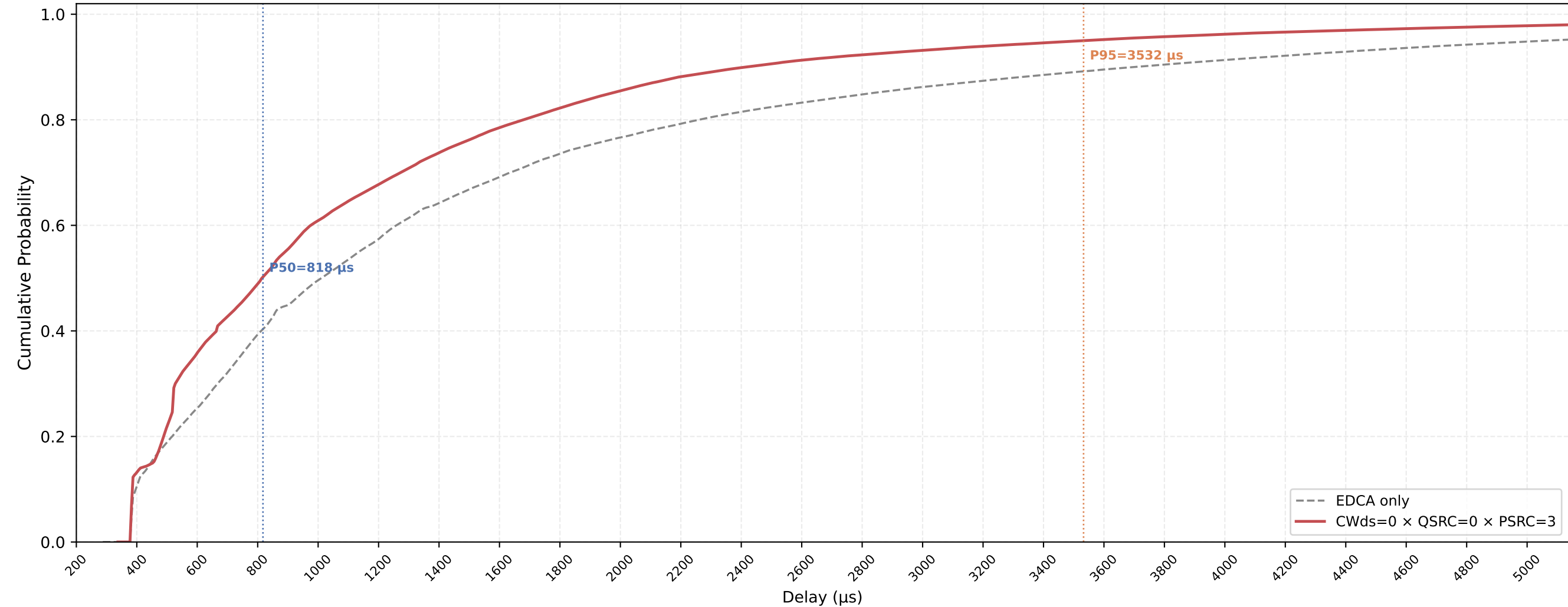
VO (all STAs) Delay CDF — CWds=0 × QSRC=0 × PSRC=3 nSta=30, nPedca=15, 0.5Mbps, avg of 10 runs
