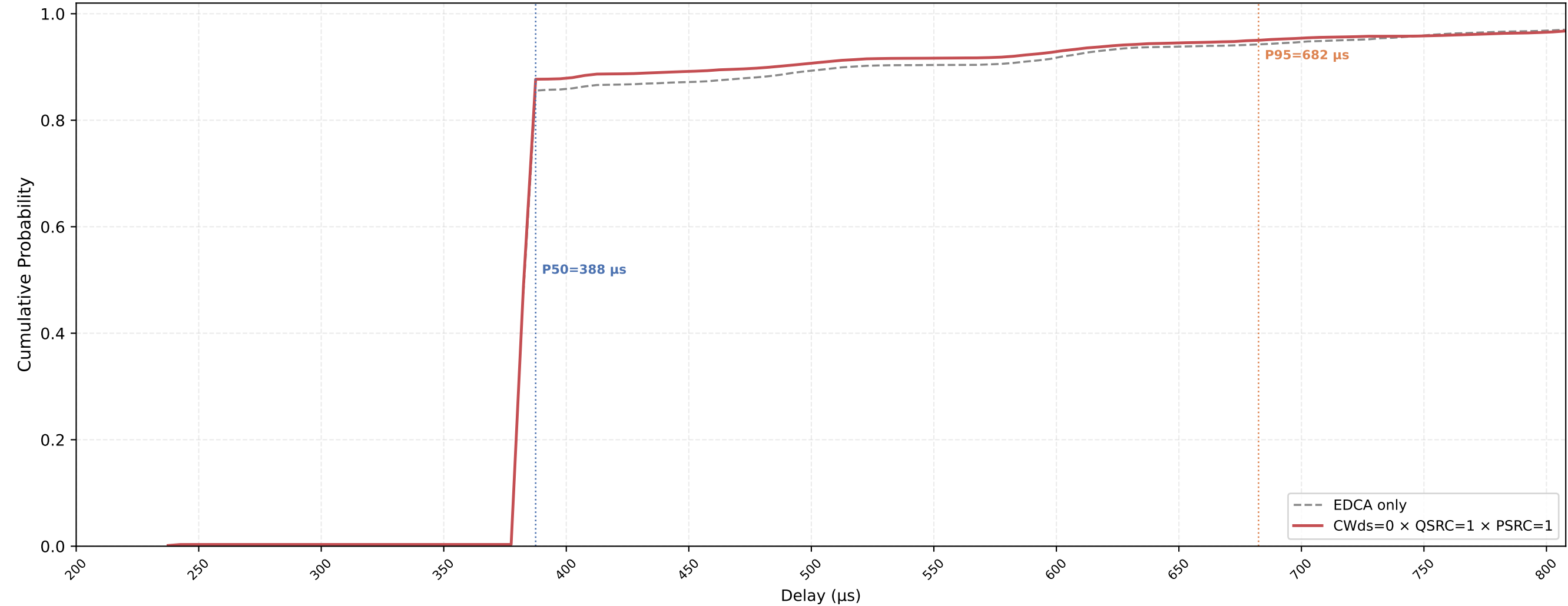
P-EDCA STA VO Delay CDF — CWds=0 × QSRC=1 × PSRC=1 nSta=30, nPedca=30, 0.1Mbps, avg of 10 runs
