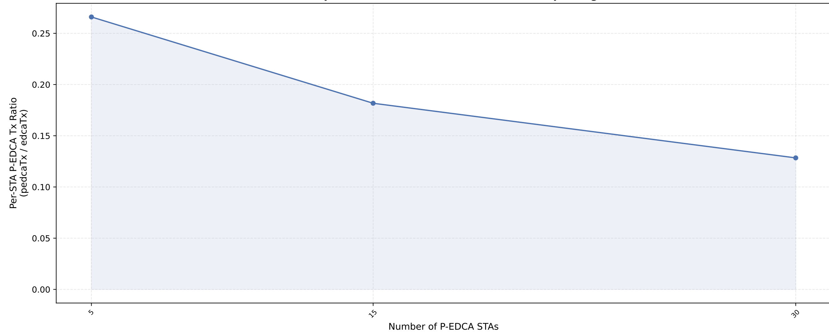
Per-P-EDCA-STA: \text{pedcaTx} / \text{edcaTx} — nSta=30, 0.5Mbps (avg of 10 runs)
