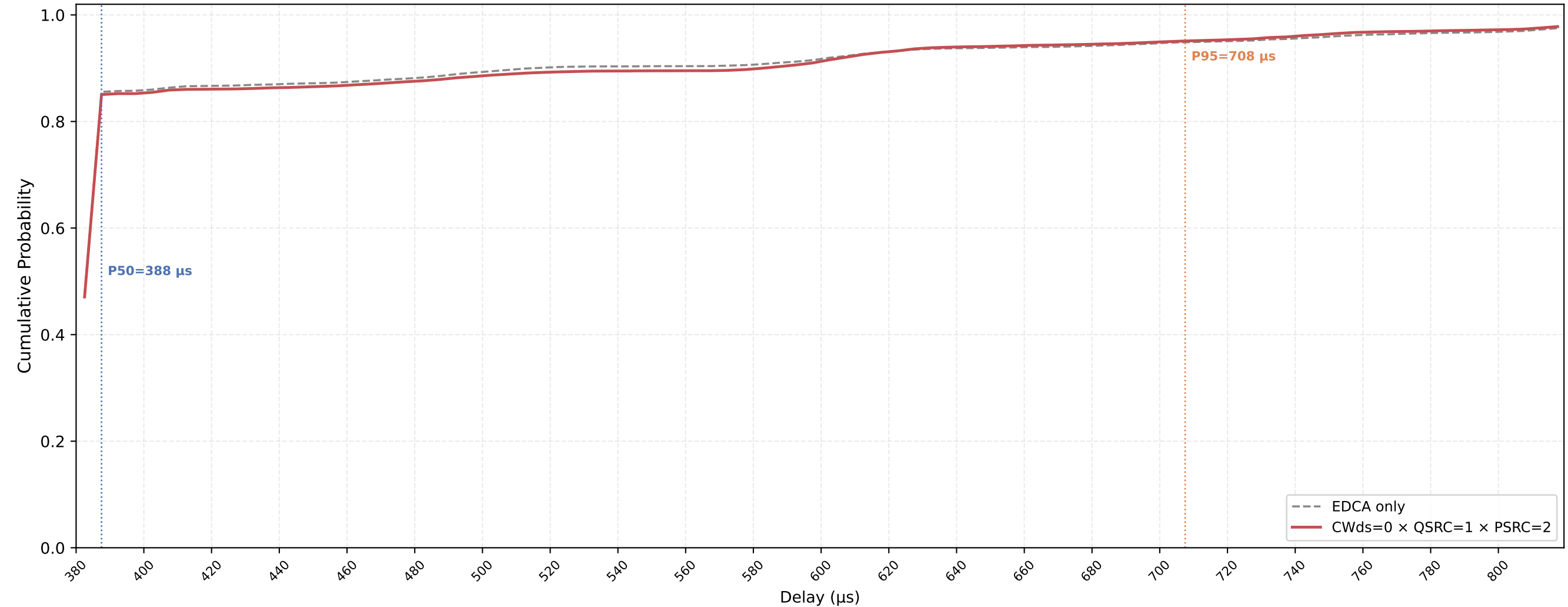
Legacy STA VO Delay CDF — CWds=0 × QSRC=1 × PSRC=2 nSta=30, nPedca=5, 0.1Mbps, avg of 10 runs
