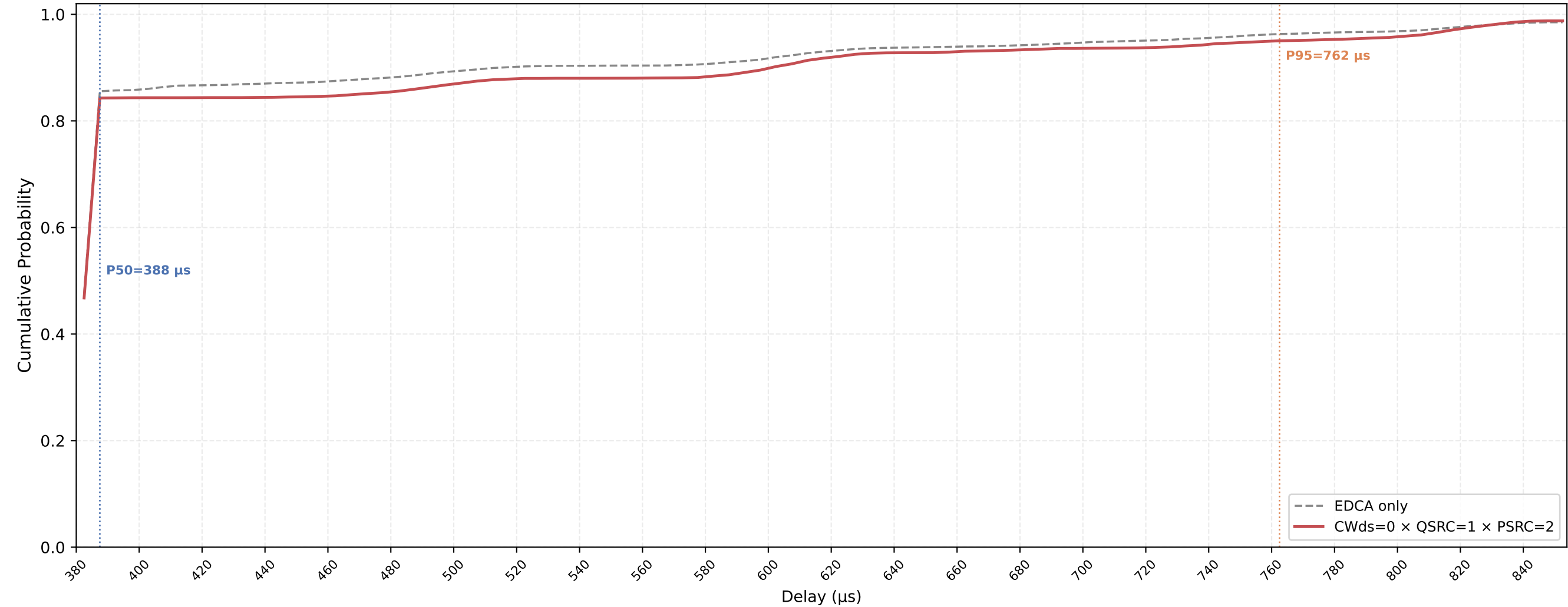
Legacy STA VO Delay CDF — CWds=0 × QSRC=1 × PSRC=2 nSta=30, nPedca=15, 0.1Mbps, avg of 10 runs
