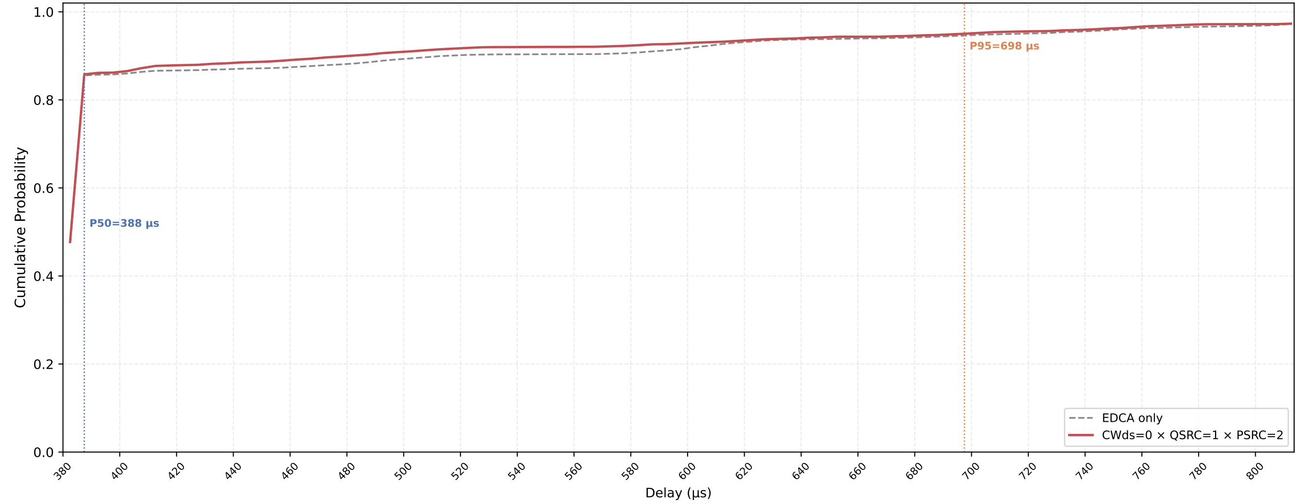
P-EDCA STA VO Delay CDF — CWds=0 × QSRC=1 × PSRC=2 nSta=30, nPedca=15, 0.1Mbps, avg of 10 runs
