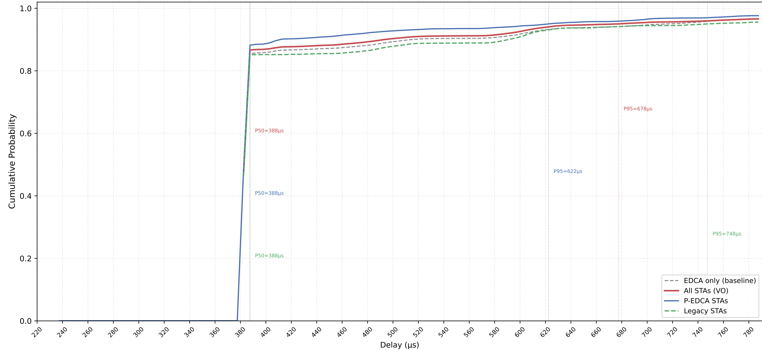
VO Delay CDF — P-EDCA / Legacy / All | CWds=0 × QSRC=2 × PSRC=1 nSta=30, nPedca=15/30, 0.1Mbps, avg of 10 runs
