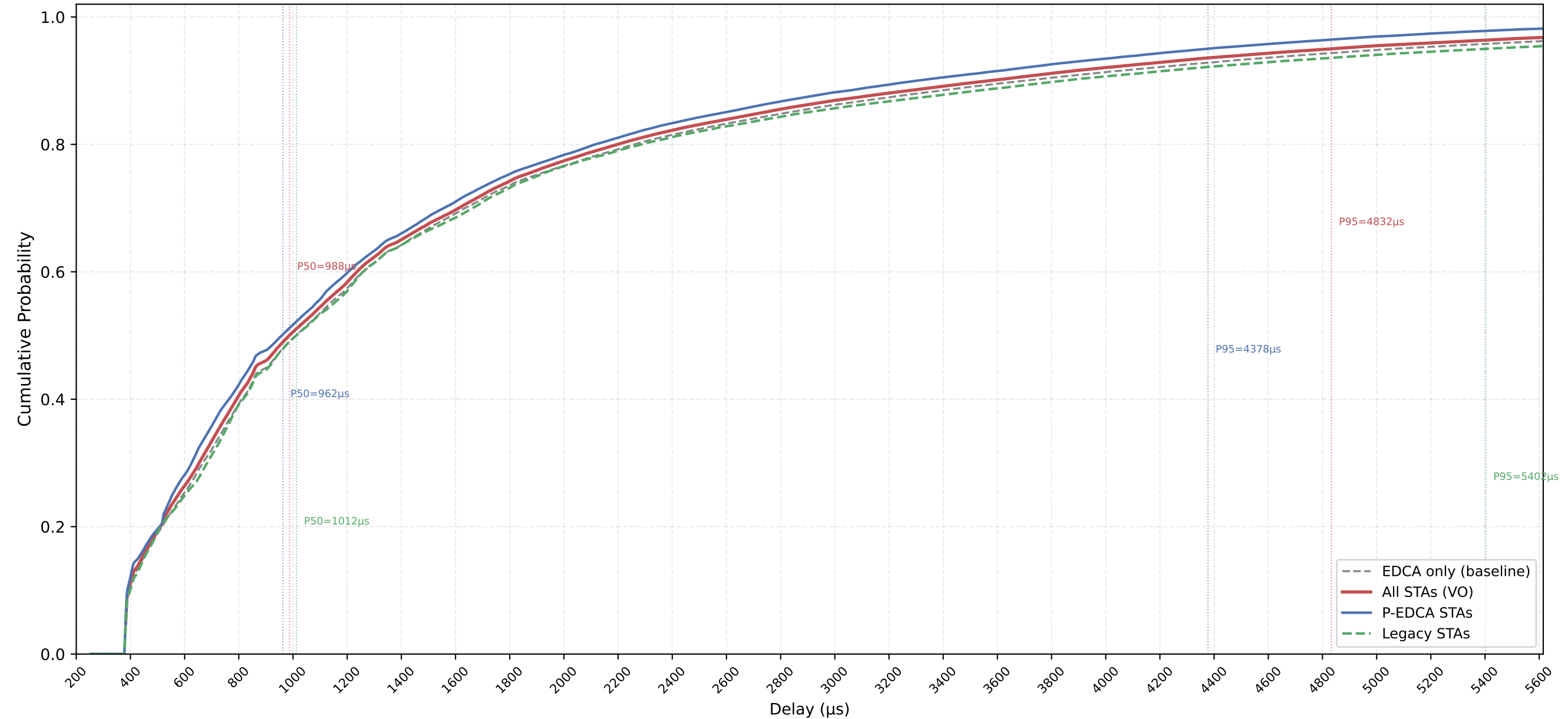
VO Delay CDF — P-EDCA / Legacy / All | CWds=0 × QSRC=2 × PSRC=1 nSta=30, nPedca=15/30, 0.5Mbps, avg of 10 runs
