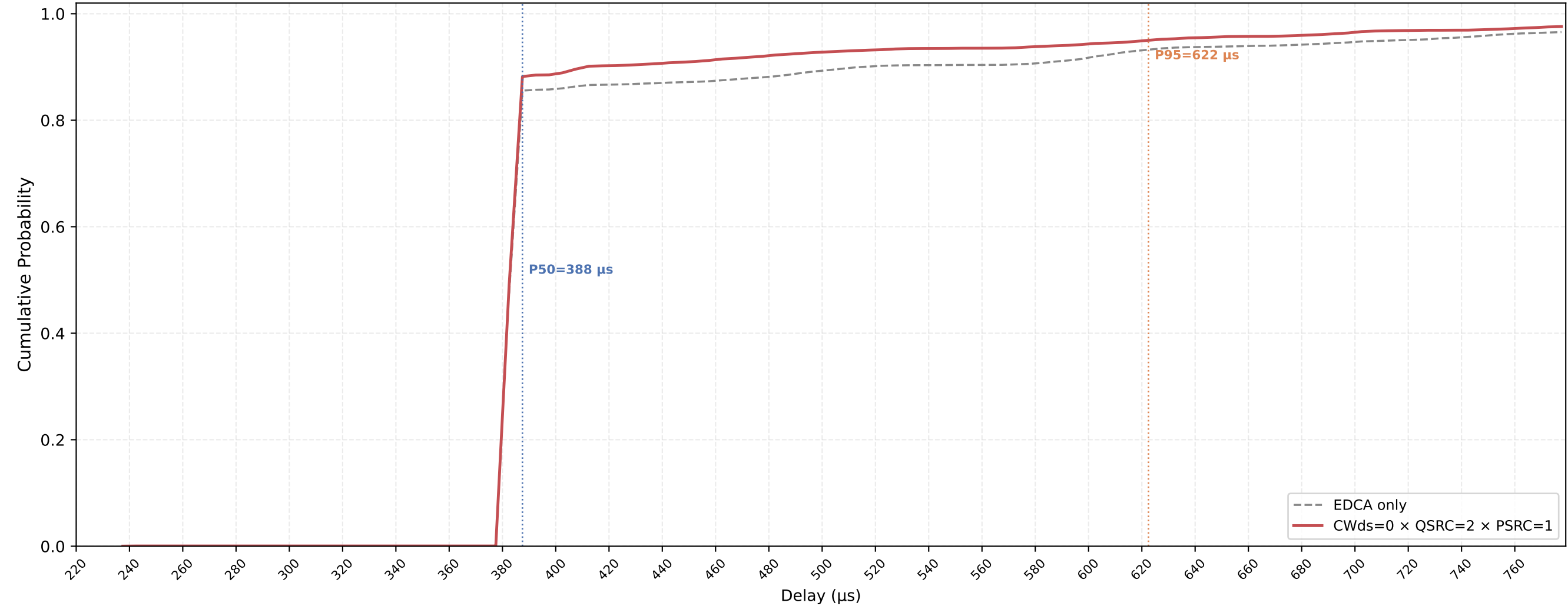
P-EDCA STA VO Delay CDF — CWds=0 × QSRC=2 × PSRC=1 nSta=30, nPedca=15, 0.1Mbps, avg of 10 runs
