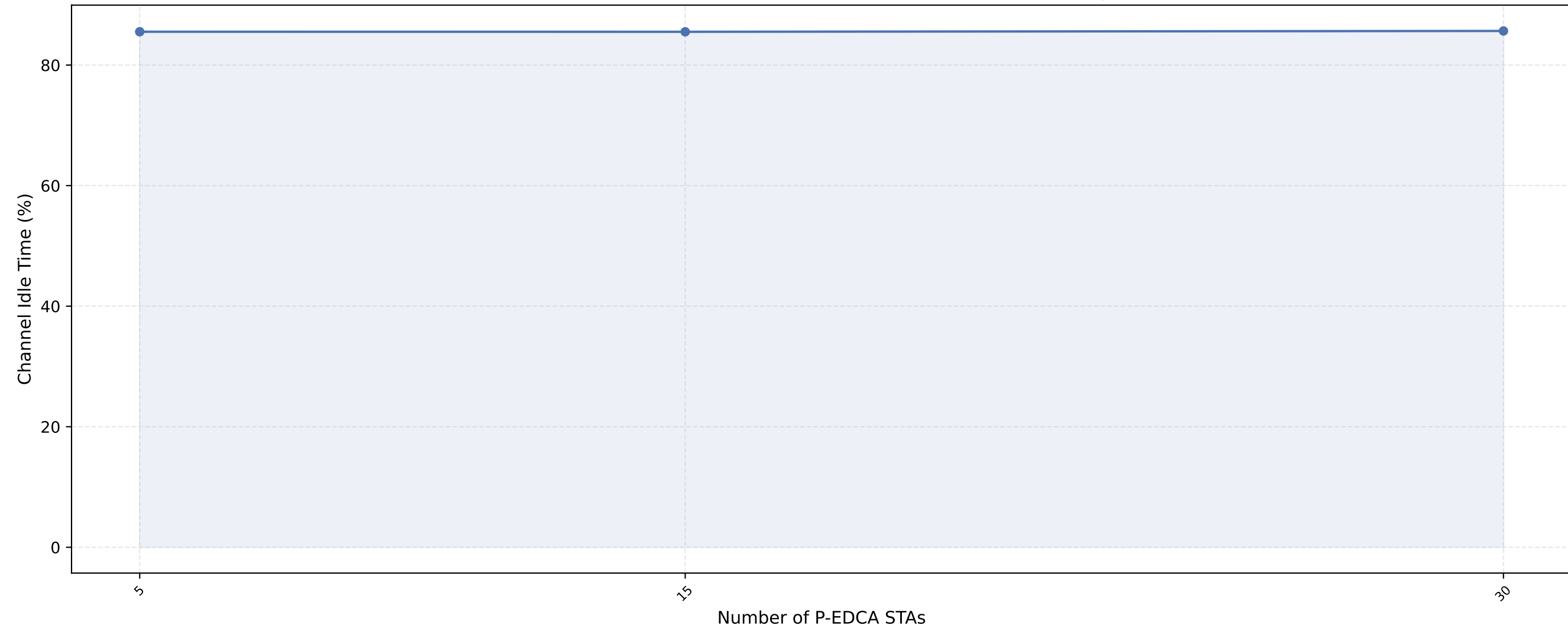
Channel Idle Time vs P-EDCA STAs — nSta=30, 0.1Mbps (avg of 10 runs)
