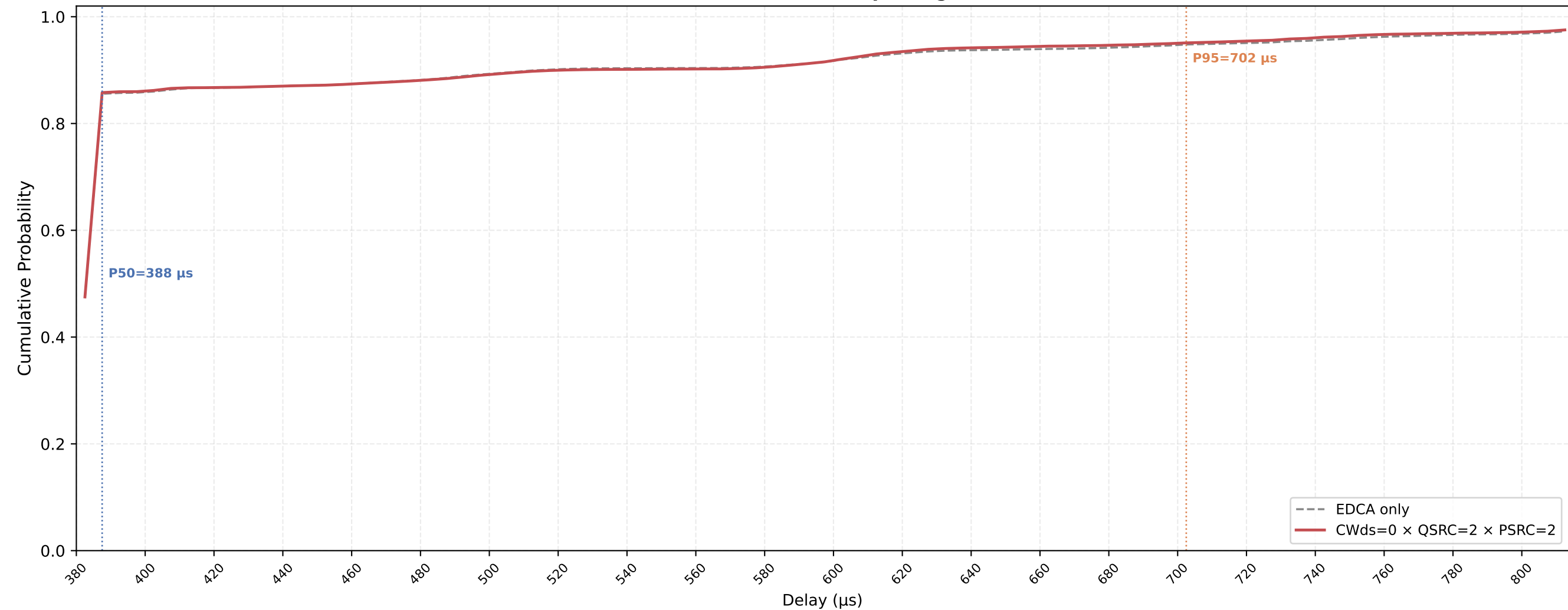
Legacy STA VO Delay CDF — CWds=0 × QSRC=2 × PSRC=2 nSta=30, nPedca=5, 0.1Mbps, avg of 10 runs
