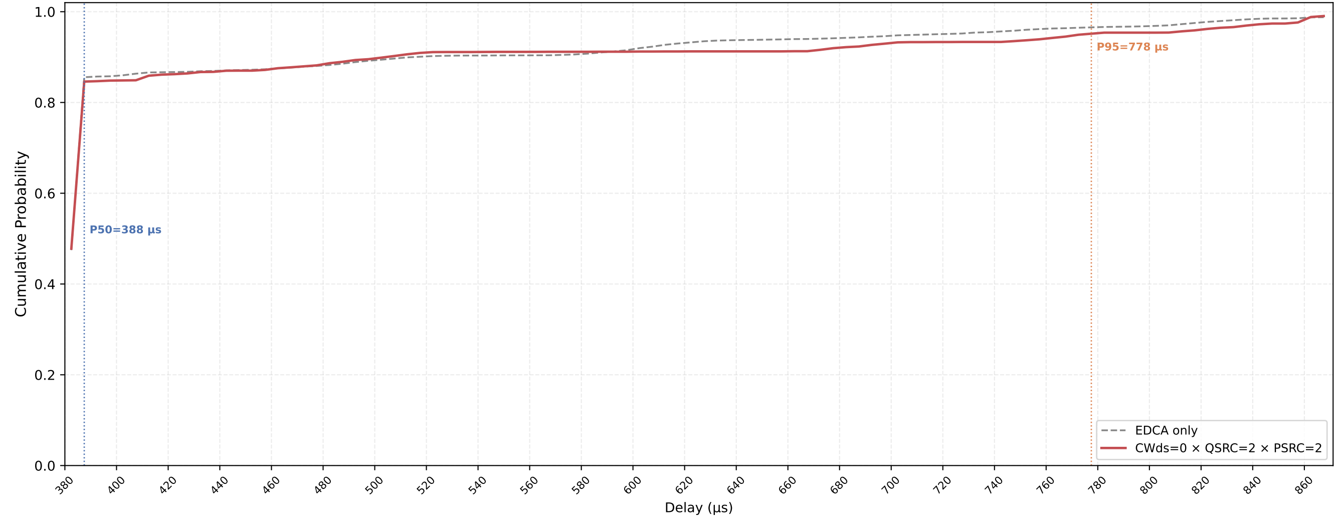
P-EDCA STA VO Delay CDF — CWds=0 × QSRC=2 × PSRC=2 nSta=30, nPedca=5, 0.1Mbps, avg of 10 runs
