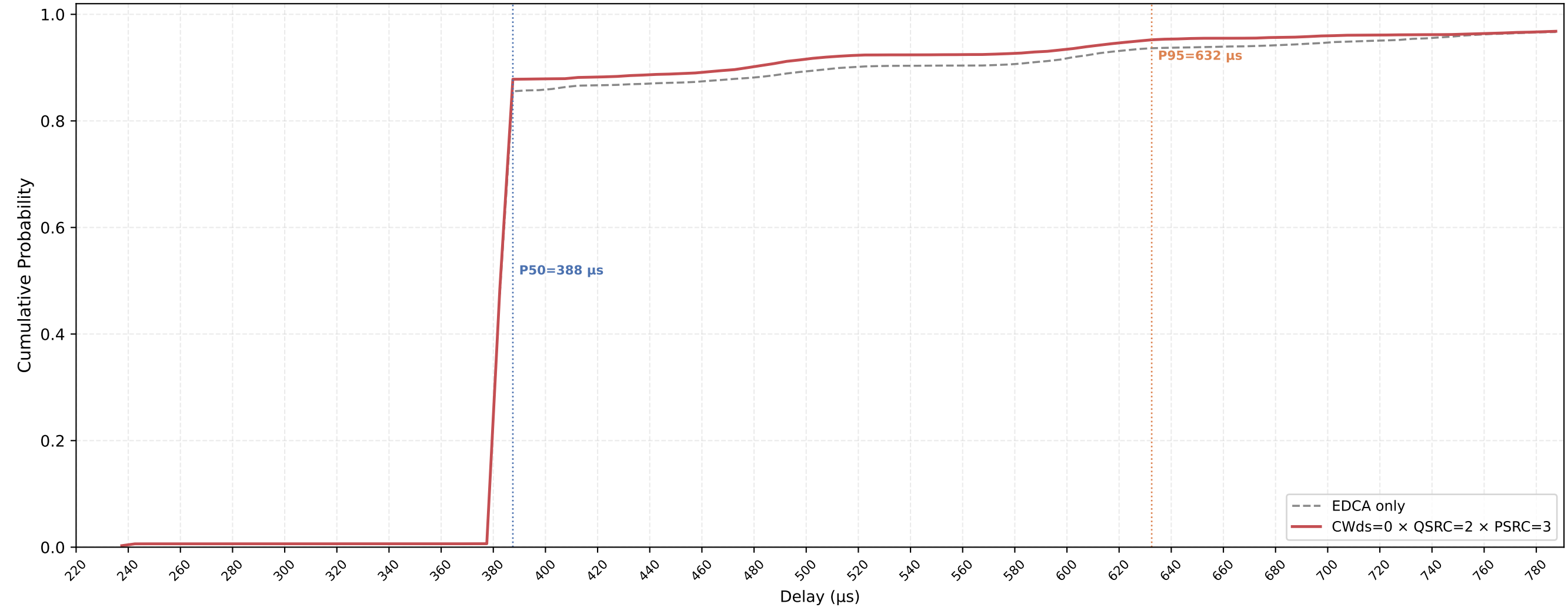
P-EDCA STA VO Delay CDF — CWds=0 × QSRC=2 × PSRC=3 nSta=30, nPedca=30, 0.1Mbps, avg of 10 runs
