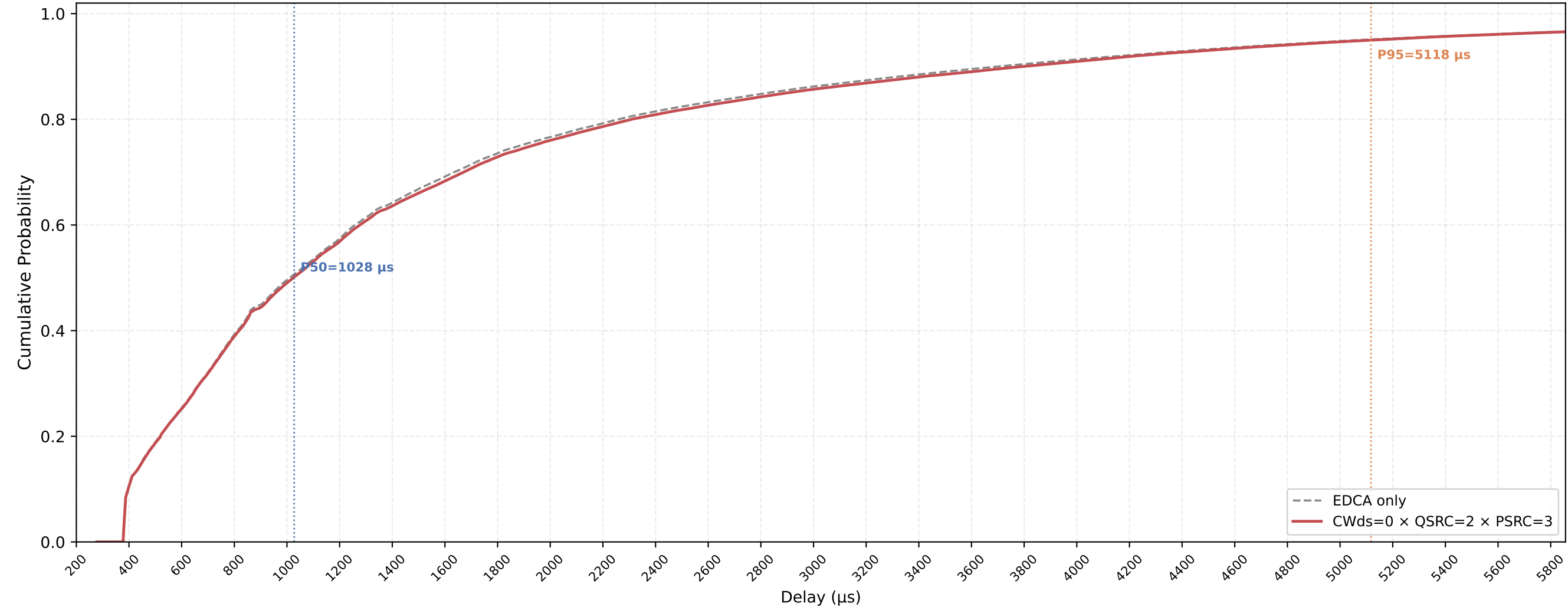
VO (all STAs) Delay CDF — CWds=0 × QSRC=2 × PSRC=3 nSta=30, nPedca=5, 0.5Mbps, avg of 10 runs
