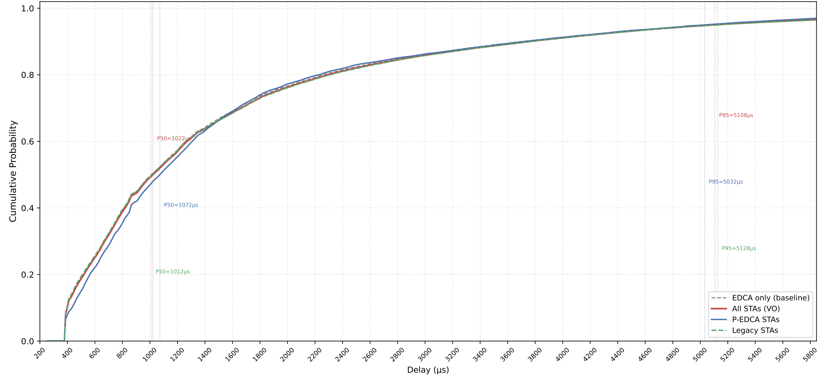
VO Delay CDF — P-EDCA / Legacy / All | CWds=0 × QSRC=3 × PSRC=1 nSta=30, nPedca=5/30, 0.5Mbps, avg of 10 runs
