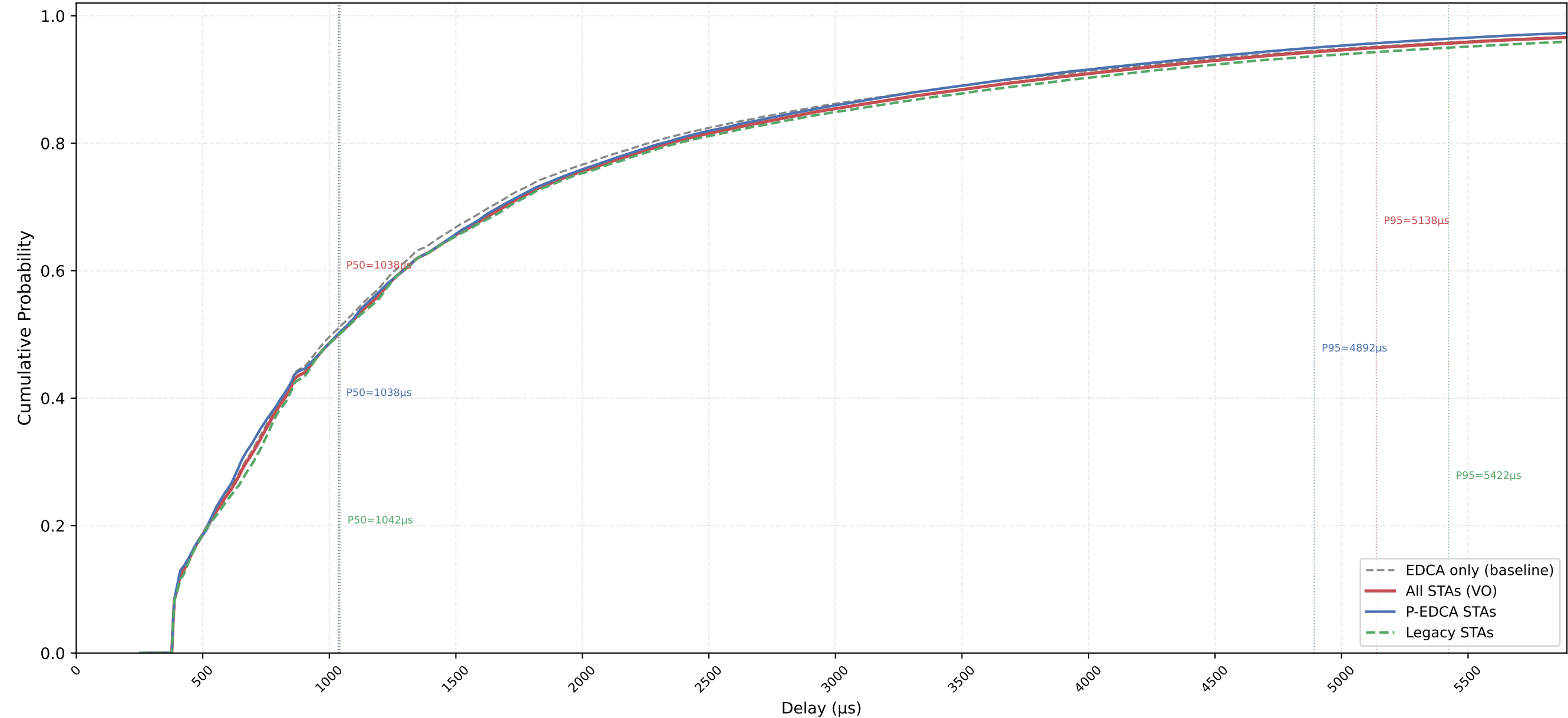
VO Delay CDF — P-EDCA / Legacy / All | CWds=0 × QSRC=3 × PSRC=1 nSta=30, nPedca=15/30, 0.5Mbps, avg of 10 runs
