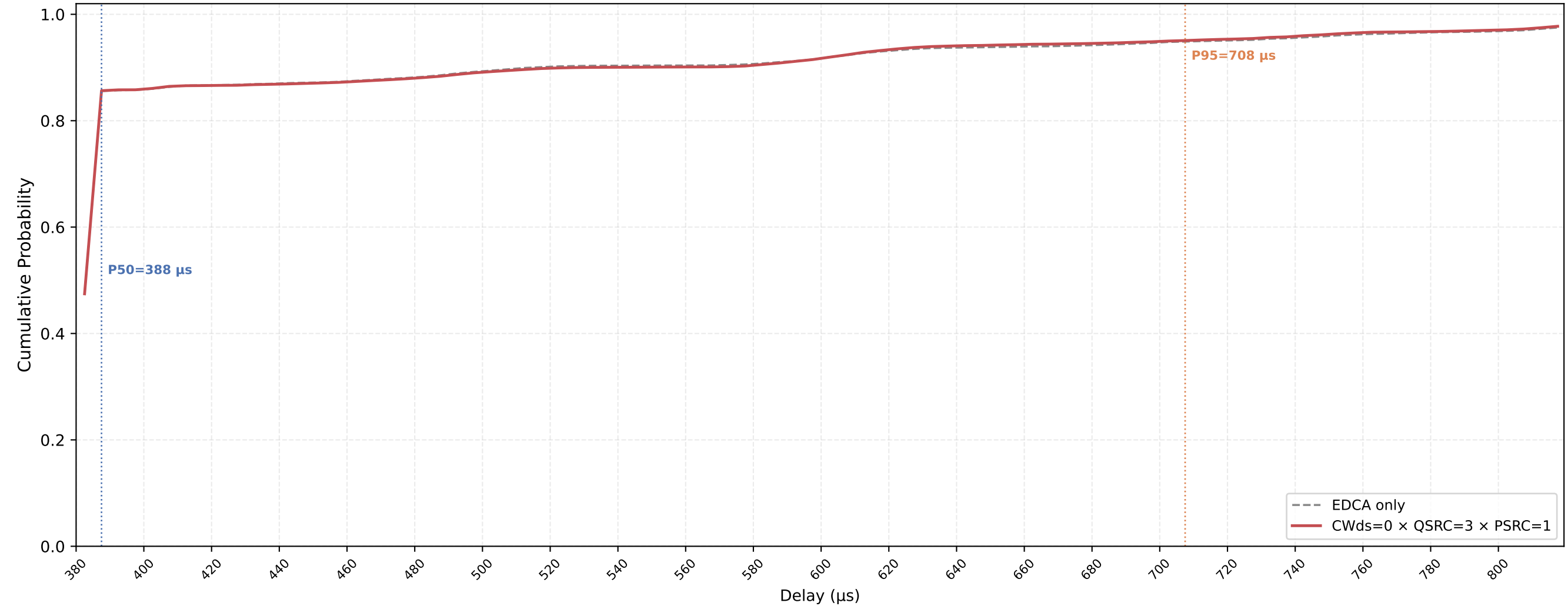
Legacy STA VO Delay CDF — CWds=0 × QSRC=3 × PSRC=1 nSta=30, nPedca=5, 0.1Mbps, avg of 10 runs
