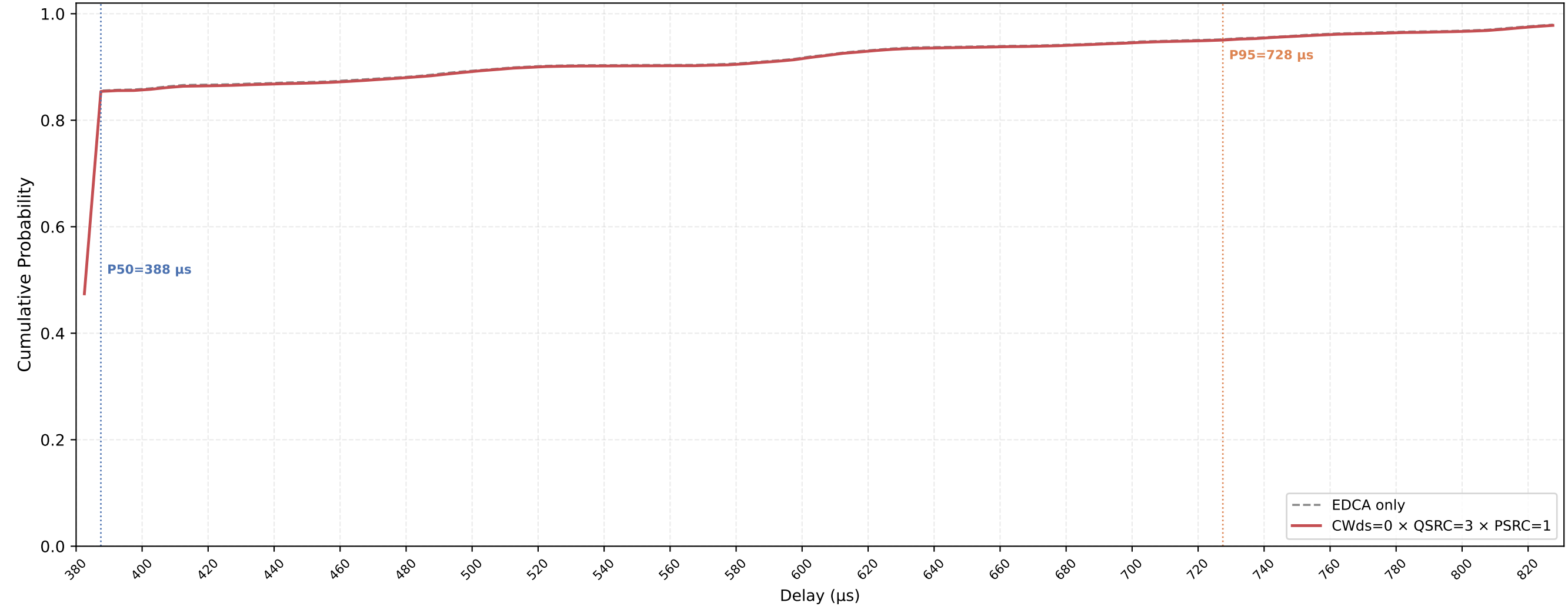
P-EDCA STA VO Delay CDF — CWds=0 × QSRC=3 × PSRC=1 nSta=30, nPedca=30, 0.1Mbps, avg of 10 runs
