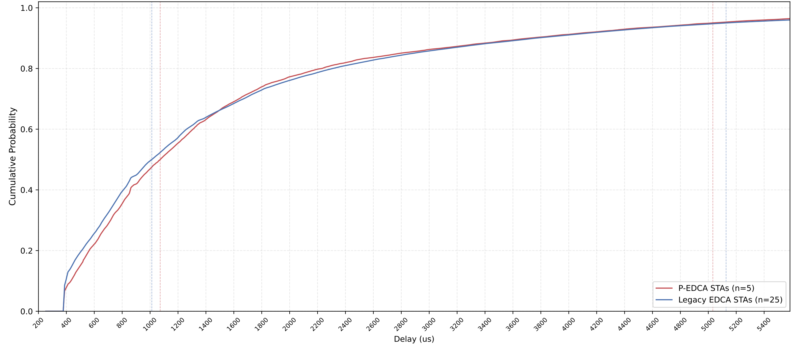
P-EDCA vs Legacy Delay CDF — n_pedca=5, n_legacy=25, nSta=30, 0.5Mbps, avg of 10 runs
