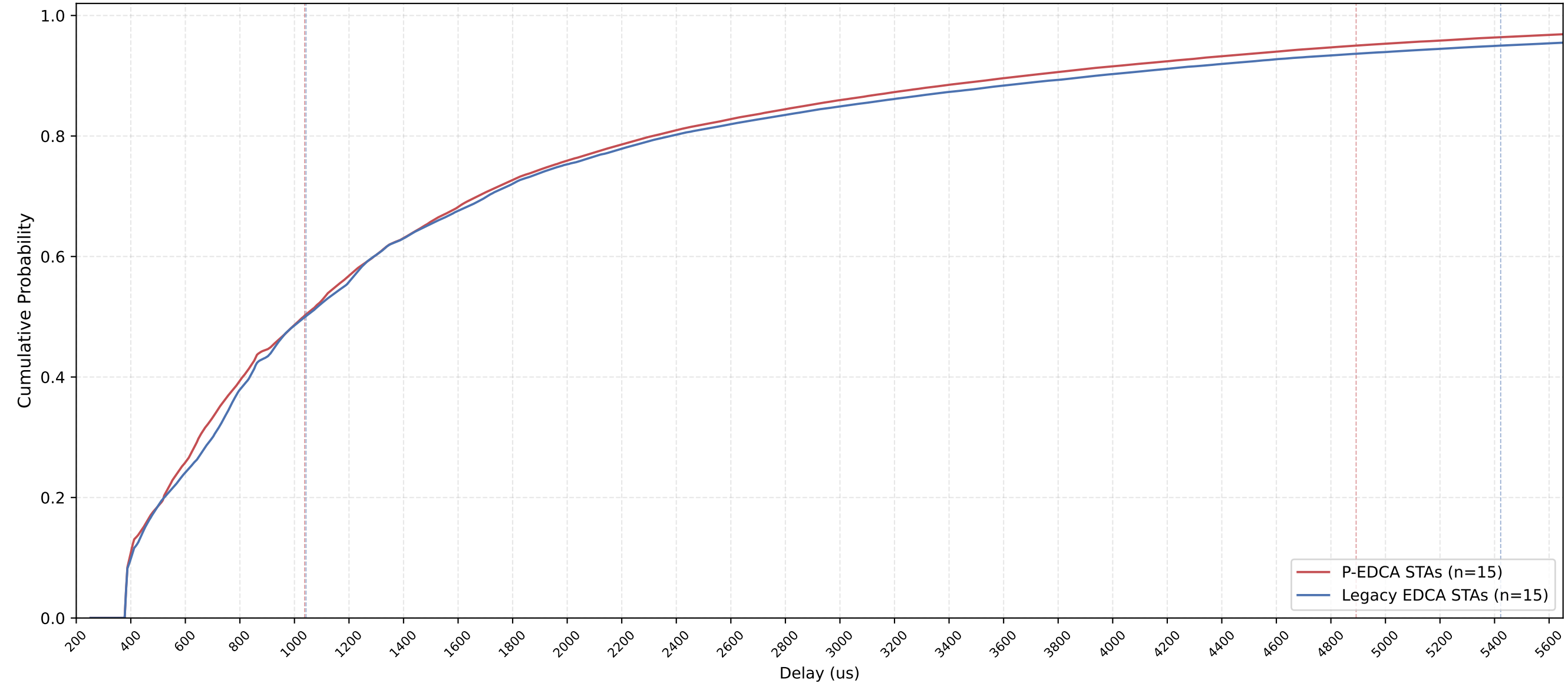
P-EDCA vs Legacy Delay CDF — n_pedca=15, n_legacy=15, nSta=30, 0.5Mbps, avg of 10 runs
