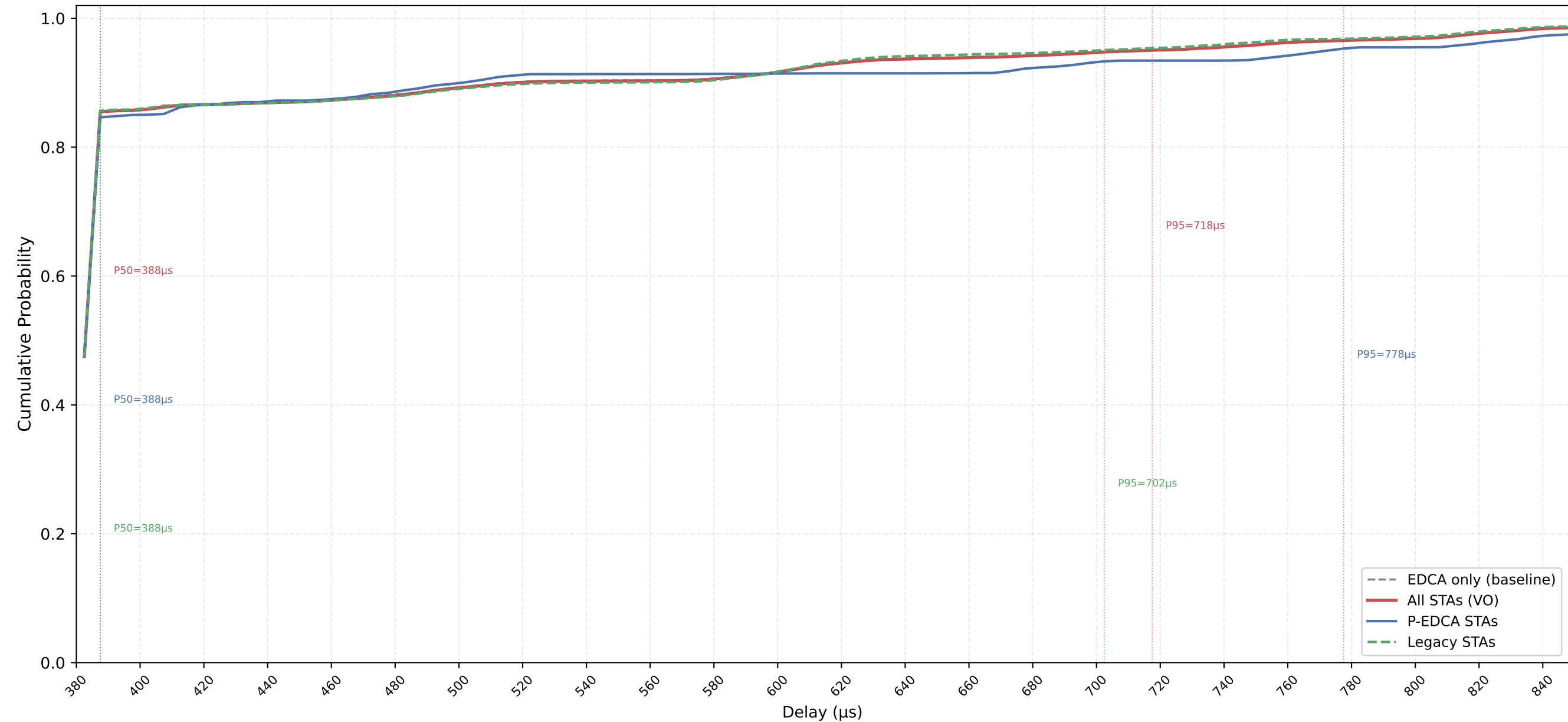
VO Delay CDF — P-EDCA / Legacy / All | CWds=0 × QSRC=3 × PSRC=2 nSta=30, nPedca=5/30, 0.1Mbps, avg of 10 runs
