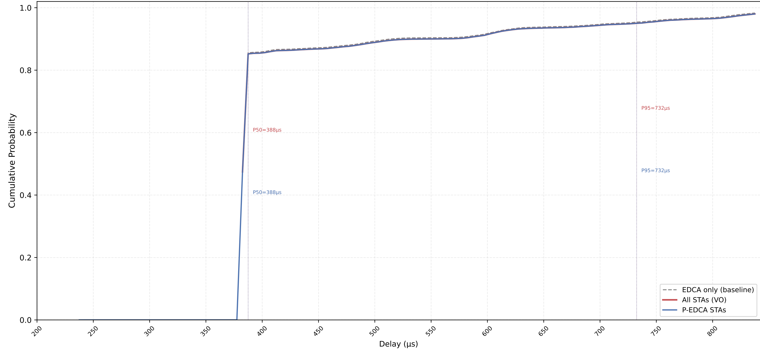
VO Delay CDF — P-EDCA / Legacy / All | CWds=0 × QSRC=3 × PSRC=2 nSta=30, nPedca=30/30, 0.1Mbps, avg of 10 runs
