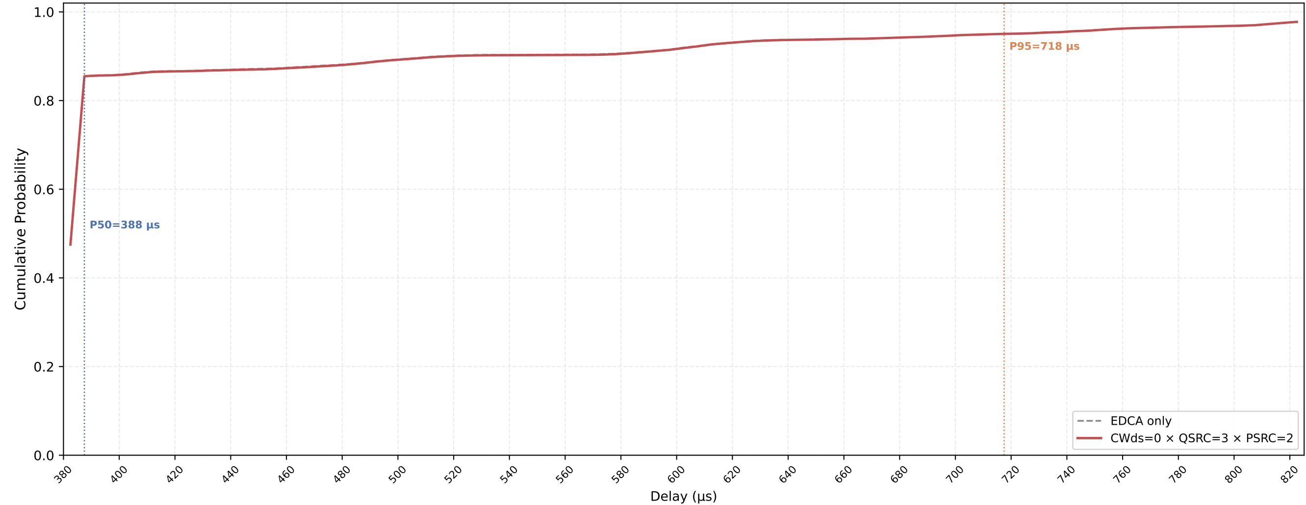
VO (all STAs) Delay CDF — CWds=0 × QSRC=3 × PSRC=2 nSta=30, nPedca=5, 0.1Mbps, avg of 10 runs
