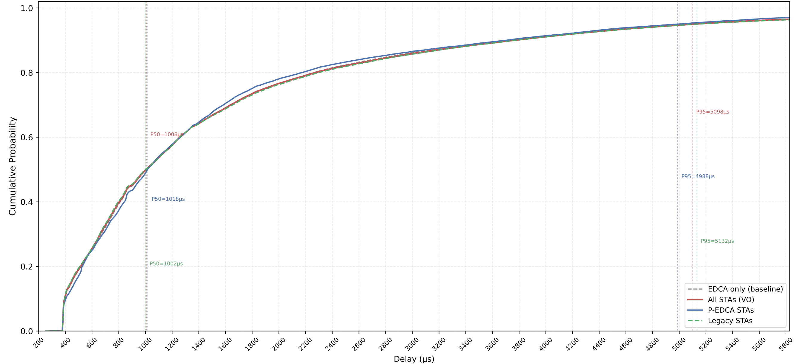
VO Delay CDF — P-EDCA / Legacy / All | CWds=0 × QSRC=3 × PSRC=3 nSta=30, nPedca=5/30, 0.5Mbps, avg of 10 runs
