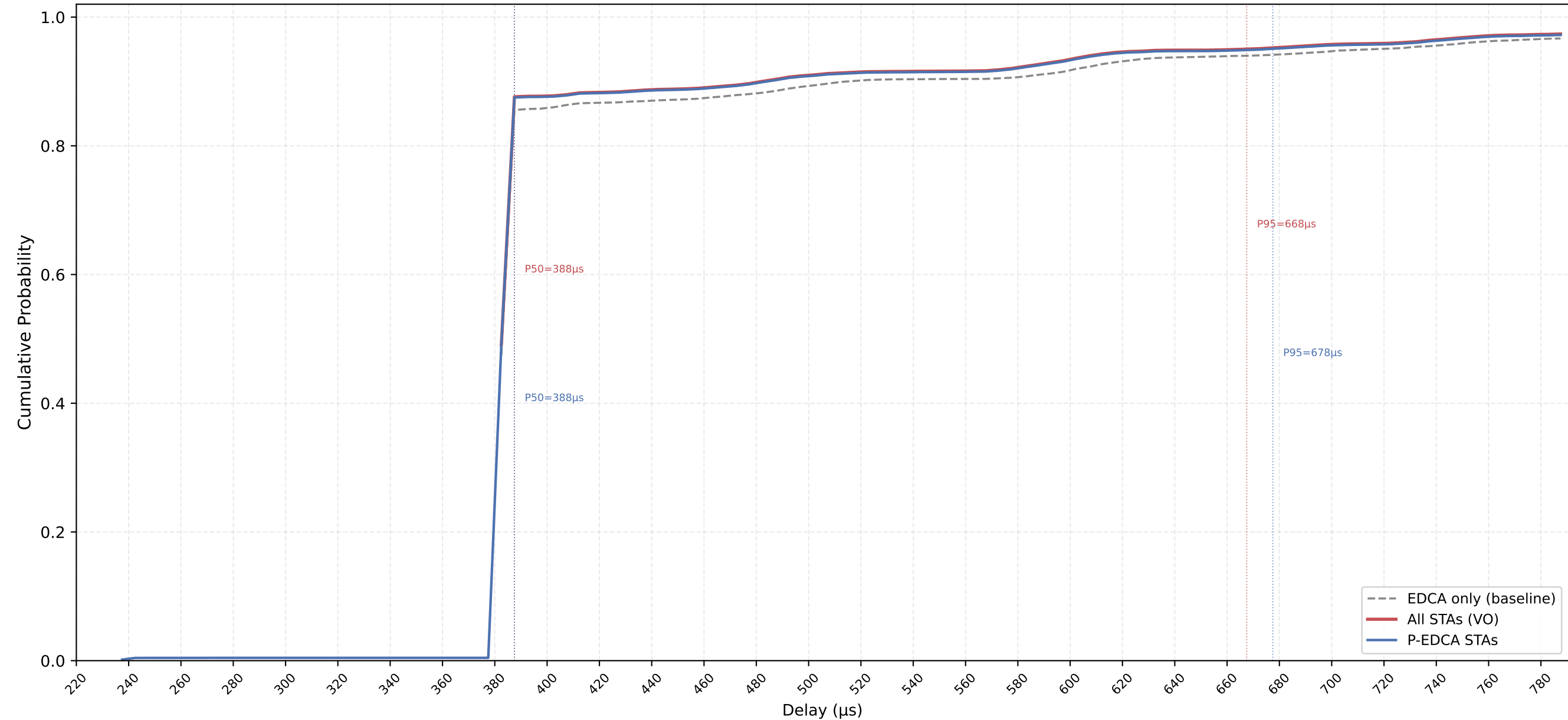
VO Delay CDF — P-EDCA / Legacy / All | CWds=0 × QSRC=3 × PSRC=3 nSta=30, nPedca=30/30, 0.1Mbps, avg of 10 runs
