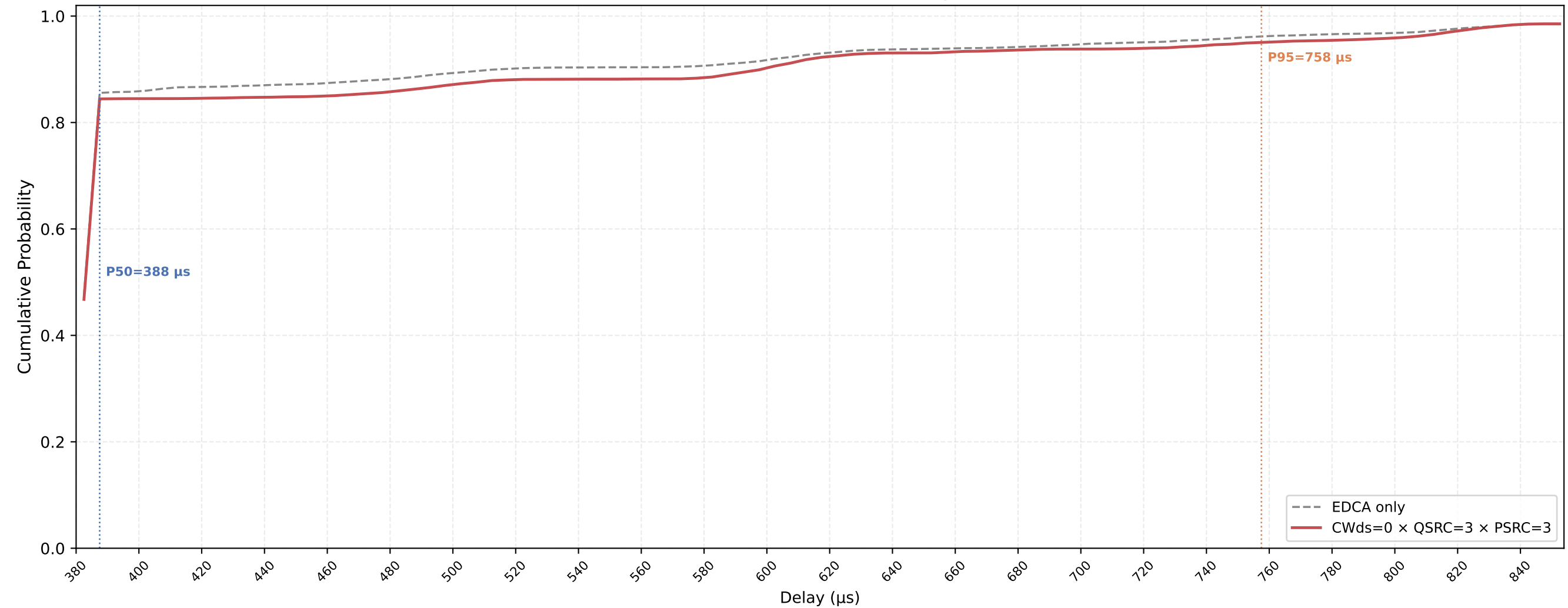
Legacy STA VO Delay CDF — CWds=0 × QSRC=3 × PSRC=3 nSta=30, nPedca=15, 0.1Mbps, avg of 10 runs
