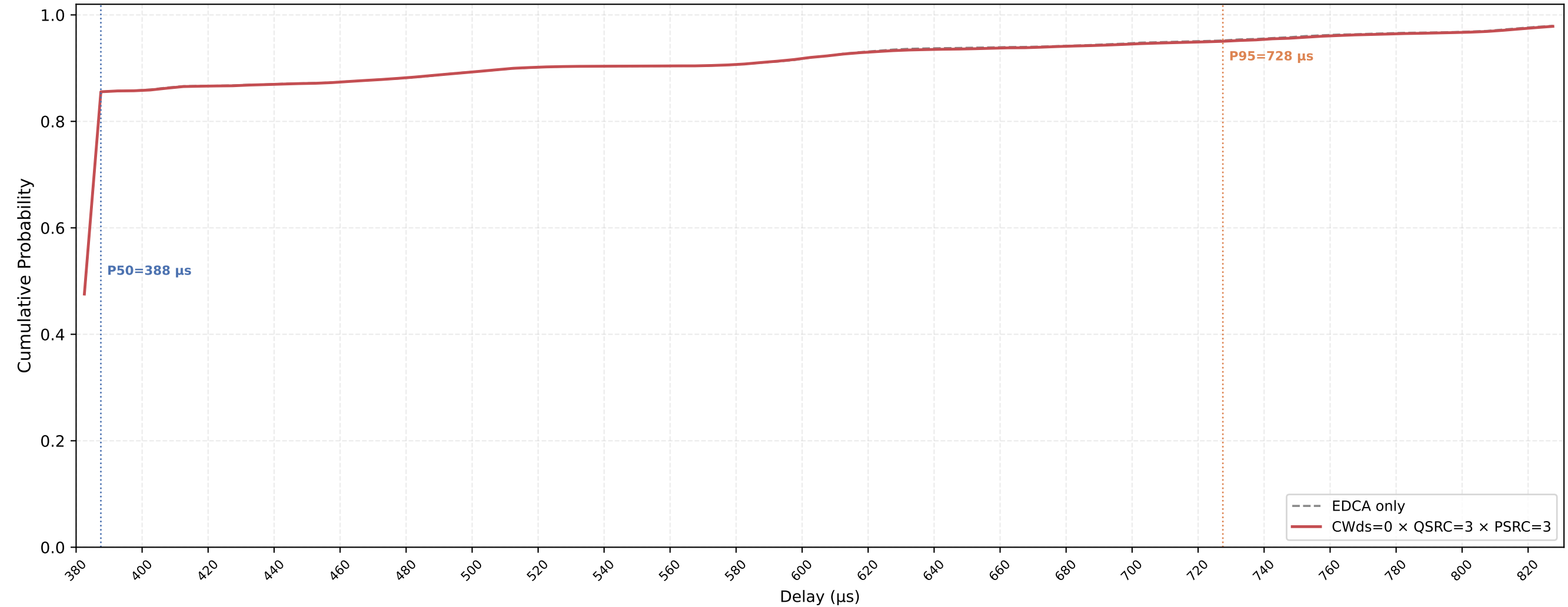
VO (all STAs) Delay CDF — CWds=0 × QSRC=3 × PSRC=3 nSta=30, nPedca=15, 0.1Mbps, avg of 10 runs
