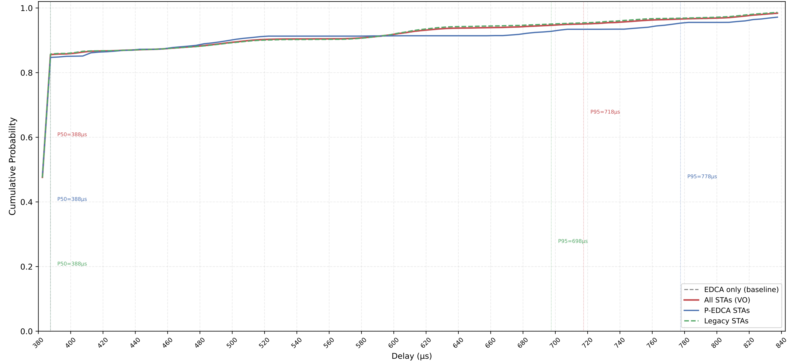
VO Delay CDF — P-EDCA / Legacy / All | CWds=0 × QSRC=4 × PSRC=1 nSta=30, nPedca=5/30, 0.1Mbps, avg of 10 runs
