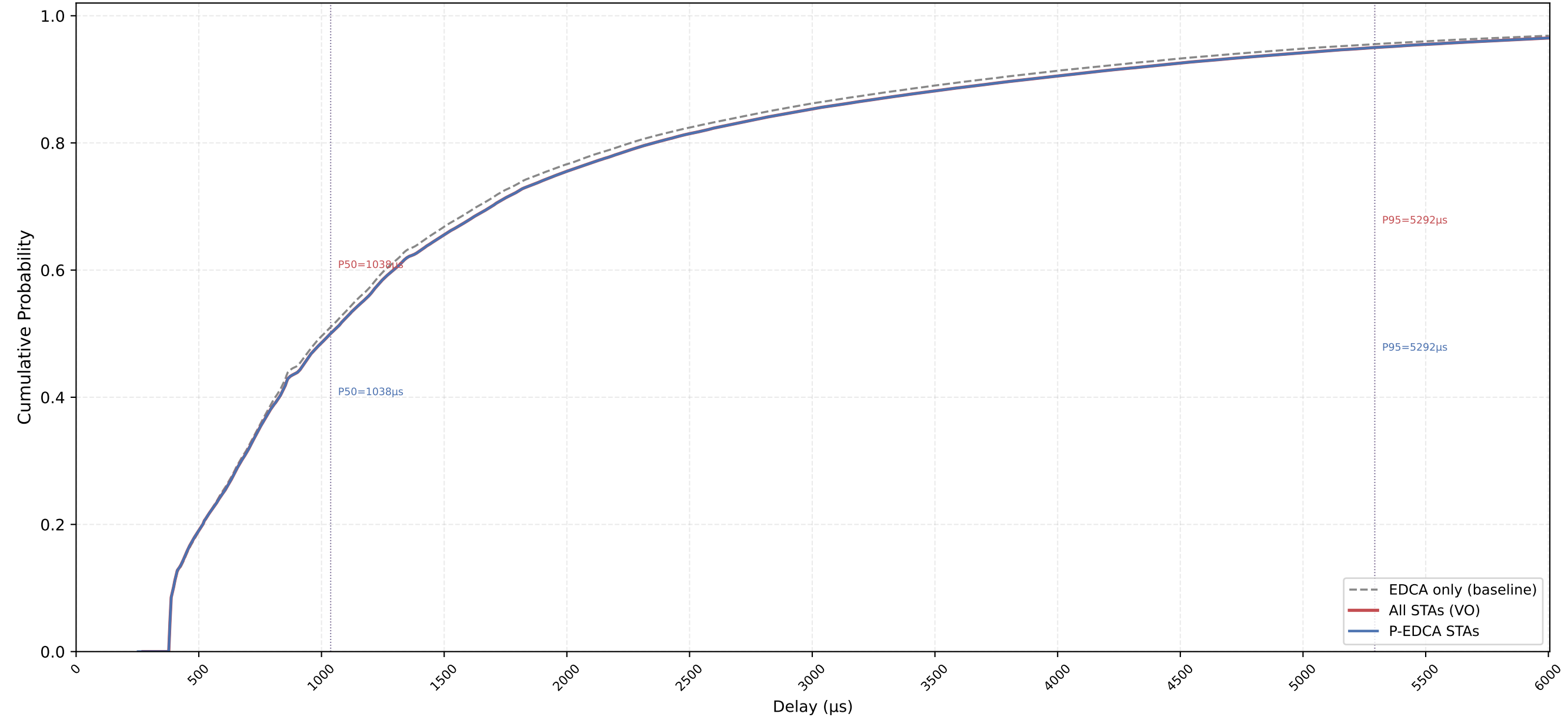
VO Delay CDF — P-EDCA / Legacy / All | CWds=0 × QSRC=4 × PSRC=1 nSta=30, nPedca=30/30, 0.5Mbps, avg of 10 runs
