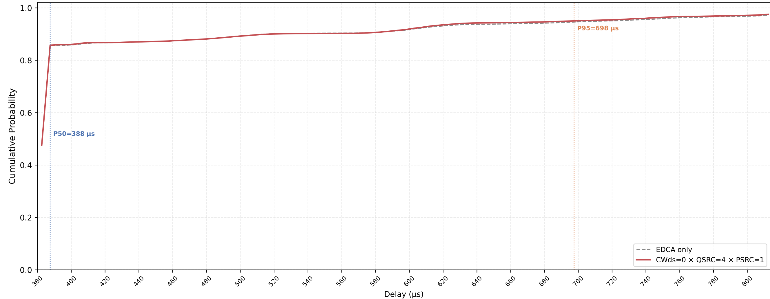
Legacy STA VO Delay CDF — CWds=0 × QSRC=4 × PSRC=1 nSta=30, nPedca=5, 0.1Mbps, avg of 10 runs
