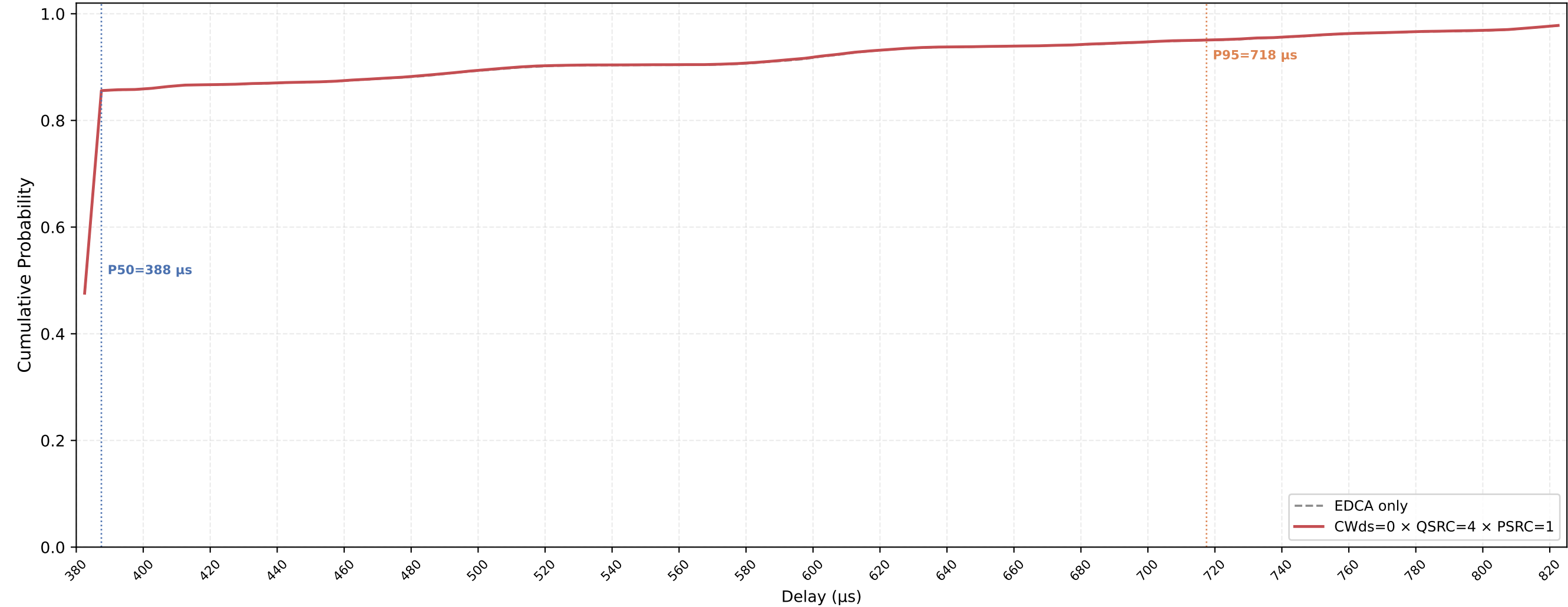
VO (all STAs) Delay CDF — CWds=0 × QSRC=4 × PSRC=1 nSta=30, nPedca=5, 0.1Mbps, avg of 10 runs
