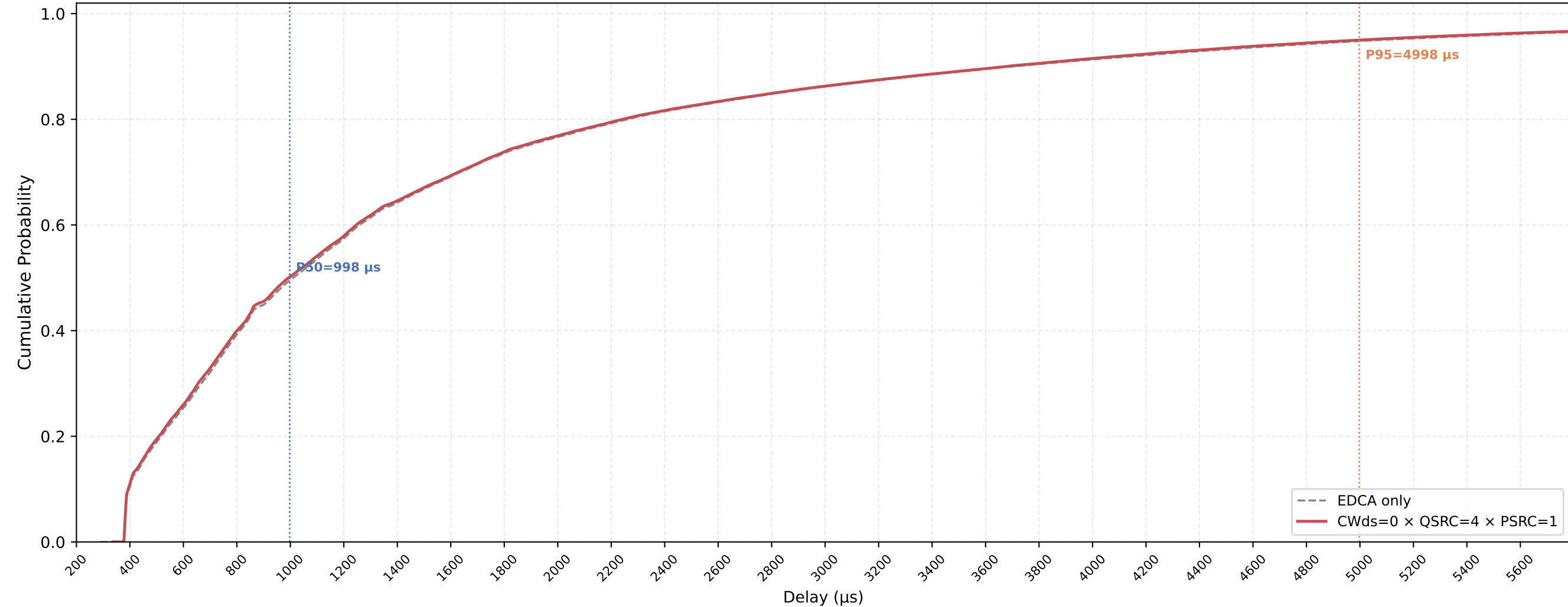
VO (all STAs) Delay CDF — CWds=0 × QSRC=4 × PSRC=1 nSta=30, nPedca=15, 0.5Mbps, avg of 10 runs
