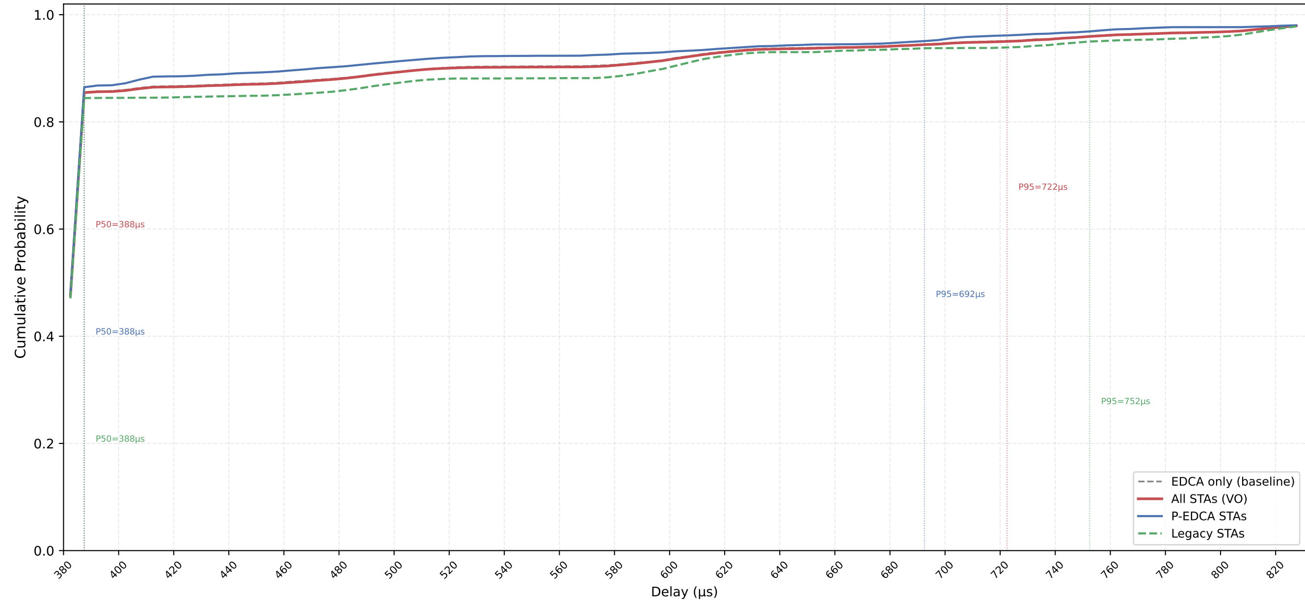
VO Delay CDF — P-EDCA / Legacy / All | CWds=0 × QSRC=4 × PSRC=2 nSta=30, nPedca=15/30, 0.1Mbps, avg of 10 runs
