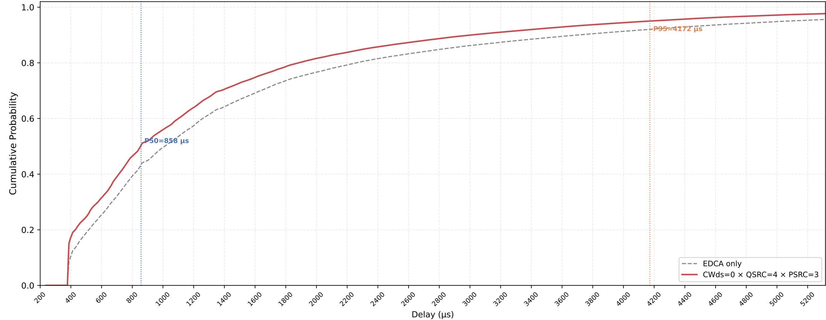
P-EDCA STA VO Delay CDF — CWds=0 × QSRC=4 × PSRC=3 nSta=30, nPedca=30, 0.5Mbps, avg of 10 runs
