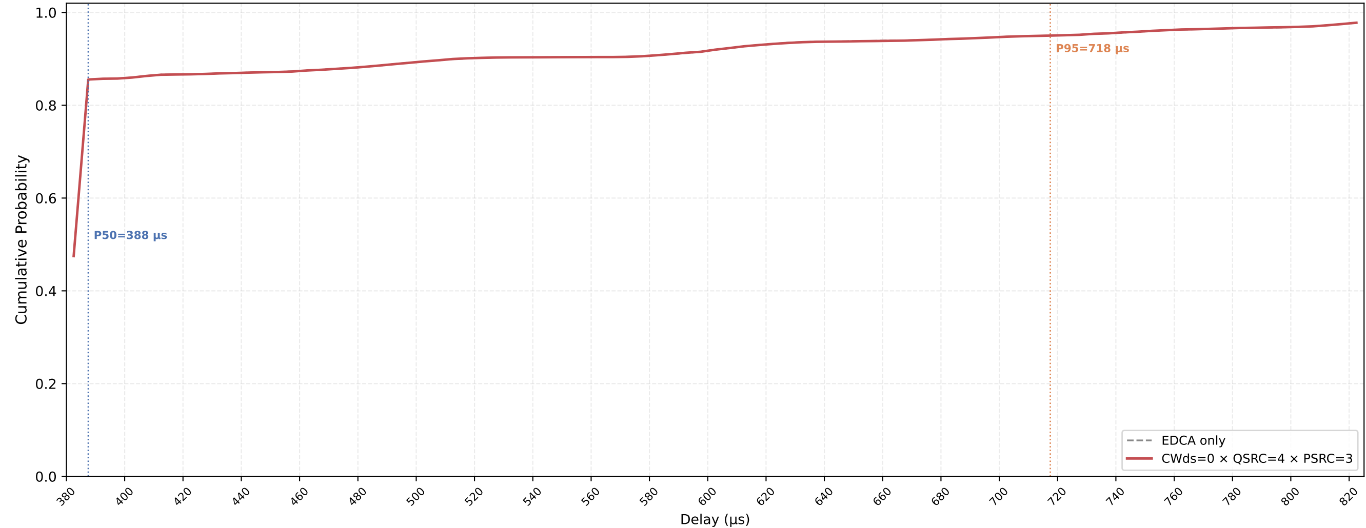
VO (all STAs) Delay CDF — CWds=0 × QSRC=4 × PSRC=3 nSta=30, nPedca=5, 0.1Mbps, avg of 10 runs
