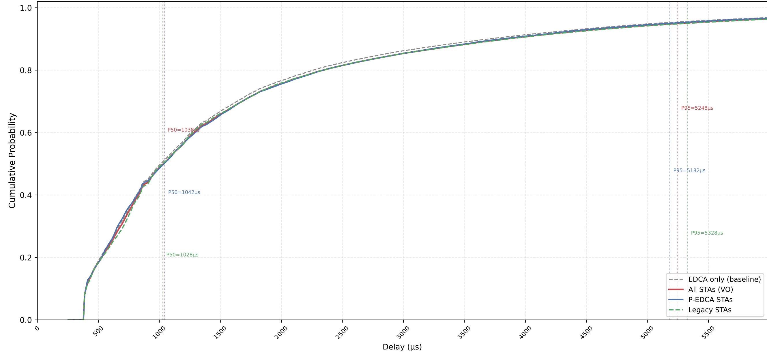
VO Delay CDF — P-EDCA / Legacy / All | CWds=0 × QSRC=5 × PSRC=1 nSta=30, nPedca=15/30, 0.5Mbps, avg of 10 runs
