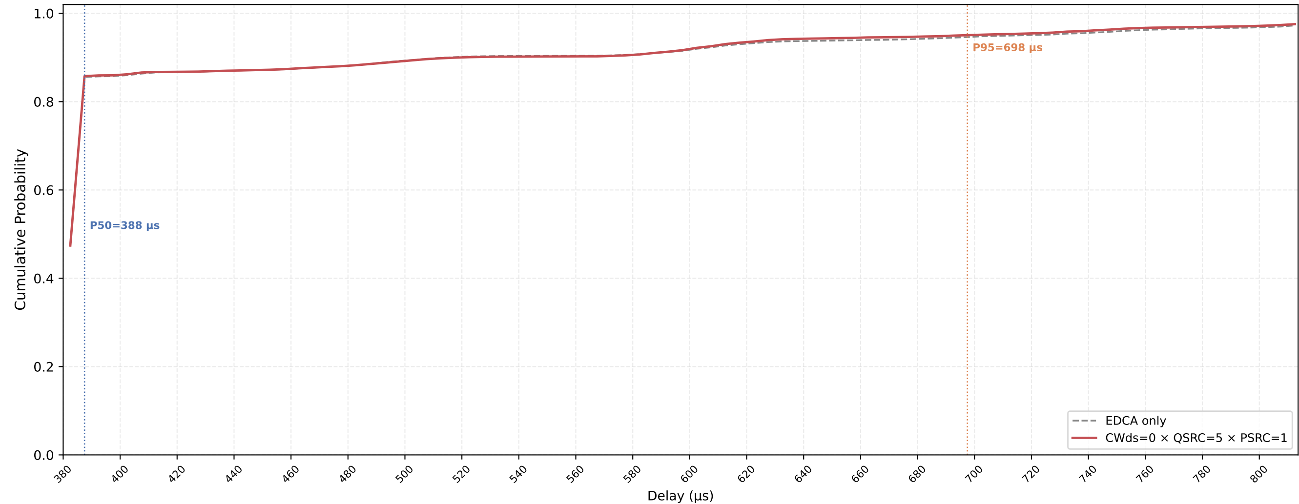
Legacy STA VO Delay CDF — CWds=0 × QSRC=5 × PSRC=1 nSta=30, nPedca=5, 0.1Mbps, avg of 10 runs
